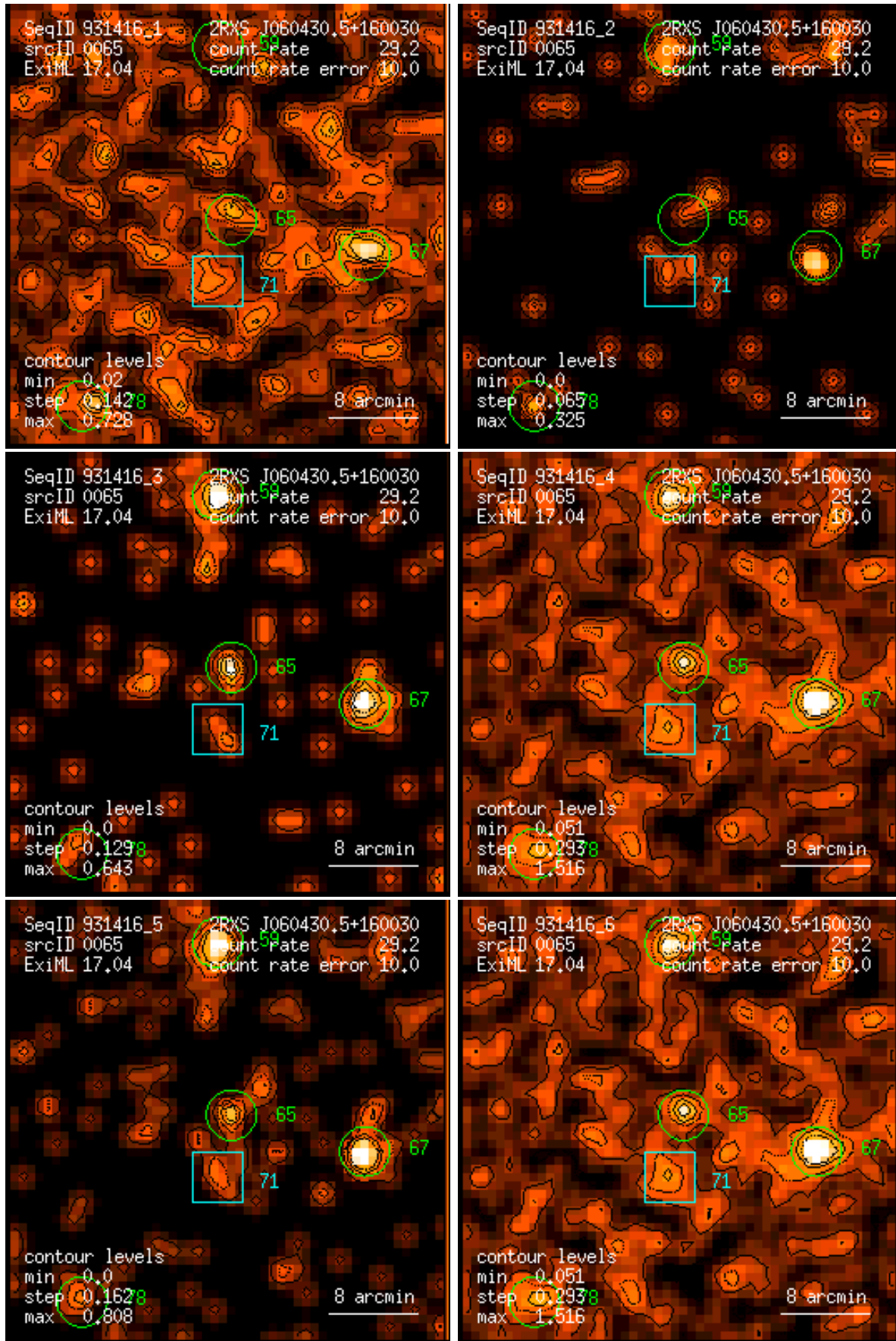
Figure 65: RASS 931416: detection 0065: band rate images, Gaussian filter: (1) PSPC channels 11 – 41, (2) 52 – 90, (3) 91 – 201, (4) 11 – 235, (5) 52 – 201, (6) 11 – 201. Broad band rates in counts/ks. Band rate contour levels in counts/ks/arcmin 2 .
