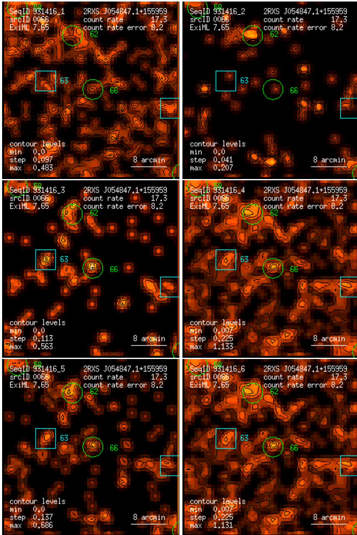
Figure 66: RASS 931416: detection 0066: band rate images, Gaussian filter: (1) PSPC channels 11 – 41, (2) 52 – 90, (3) 91 – 201, (4) 11 – 235, (5) 52 – 201, (6) 11 – 201. Broad band rates in counts/ks. Band rate contour levels in counts/ks/arcmin 2 .
