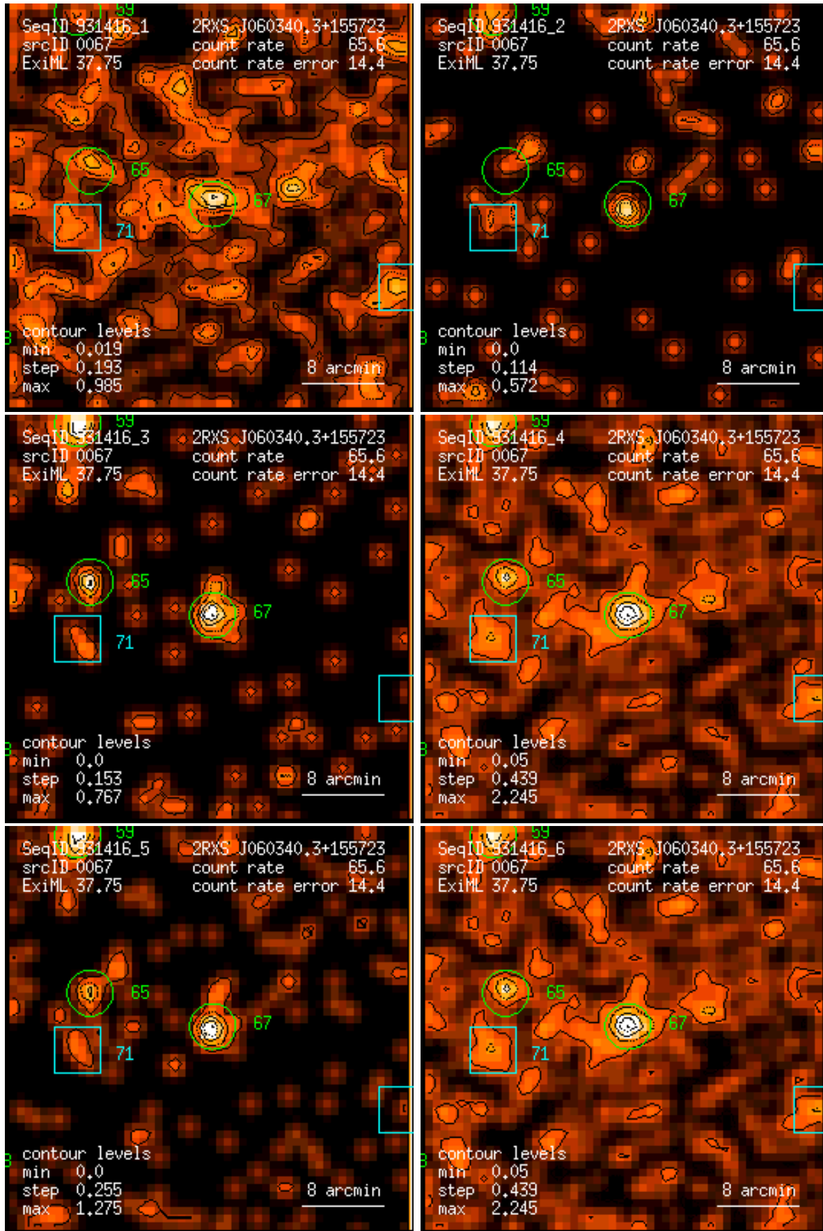
Figure 67: RASS 931416: detection 0067: band rate images, Gaussian filter: (1) PSPC channels 11 – 41, (2) 52 – 90, (3) 91 – 201, (4) 11 – 235, (5) 52 – 201, (6) 11 – 201. Broad band rates in counts/ks. Band rate contour levels in counts/ks/arcmin 2 .
