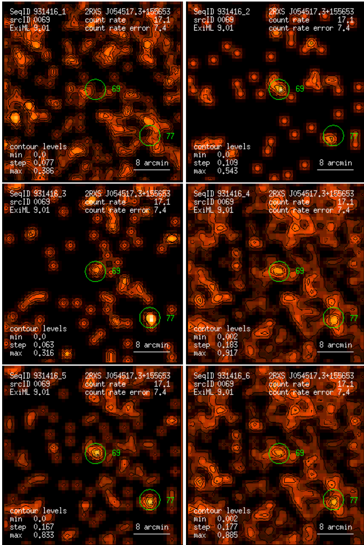
Figure 69: RASS 931416: detection 0069: band rate images, Gaussian filter: (1) PSPC channels 11 – 41, (2) 52 – 90, (3) 91 – 201, (4) 11 – 235, (5) 52 – 201, (6) 11 – 201. Broad band rates in counts/ks. Band rate contour levels in counts/ks/arcmin 2 .
