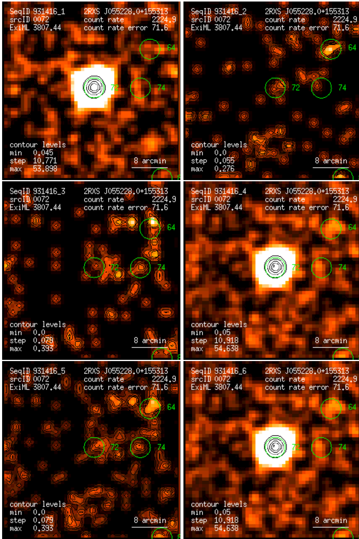
Figure 72: RASS 931416: detection 0072: band rate images, Gaussian filter: (1) PSPC channels 11 – 41, (2) 52 – 90, (3) 91 – 201, (4) 11 – 235, (5) 52 – 201, (6) 11 – 201. Broad band rates in counts/ks. Band rate contour levels in counts/ks/arcmin 2 .
