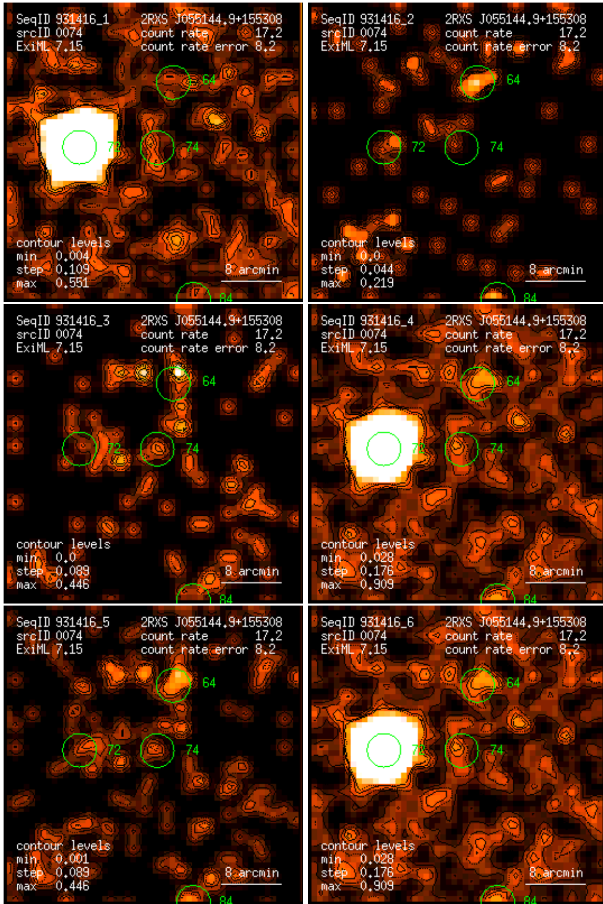
Figure 74: RASS 931416: detection 0074: band rate images, Gaussian filter: (1) PSPC channels 11 – 41, (2) 52 – 90, (3) 91 – 201, (4) 11 – 235, (5) 52 – 201, (6) 11 – 201. Broad band rates in counts/ks. Band rate contour levels in counts/ks/arcmin 2 .
