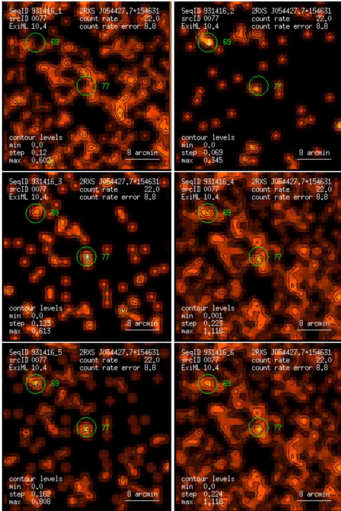
Figure 77: RASS 931416: detection 0077: band rate images, Gaussian filter: (1) PSPC channels 11 – 41, (2) 52 – 90, (3) 91 – 201, (4) 11 – 235, (5) 52 – 201, (6) 11 – 201. Broad band rates in counts/ks. Band rate contour levels in counts/ks/arcmin 2 .
