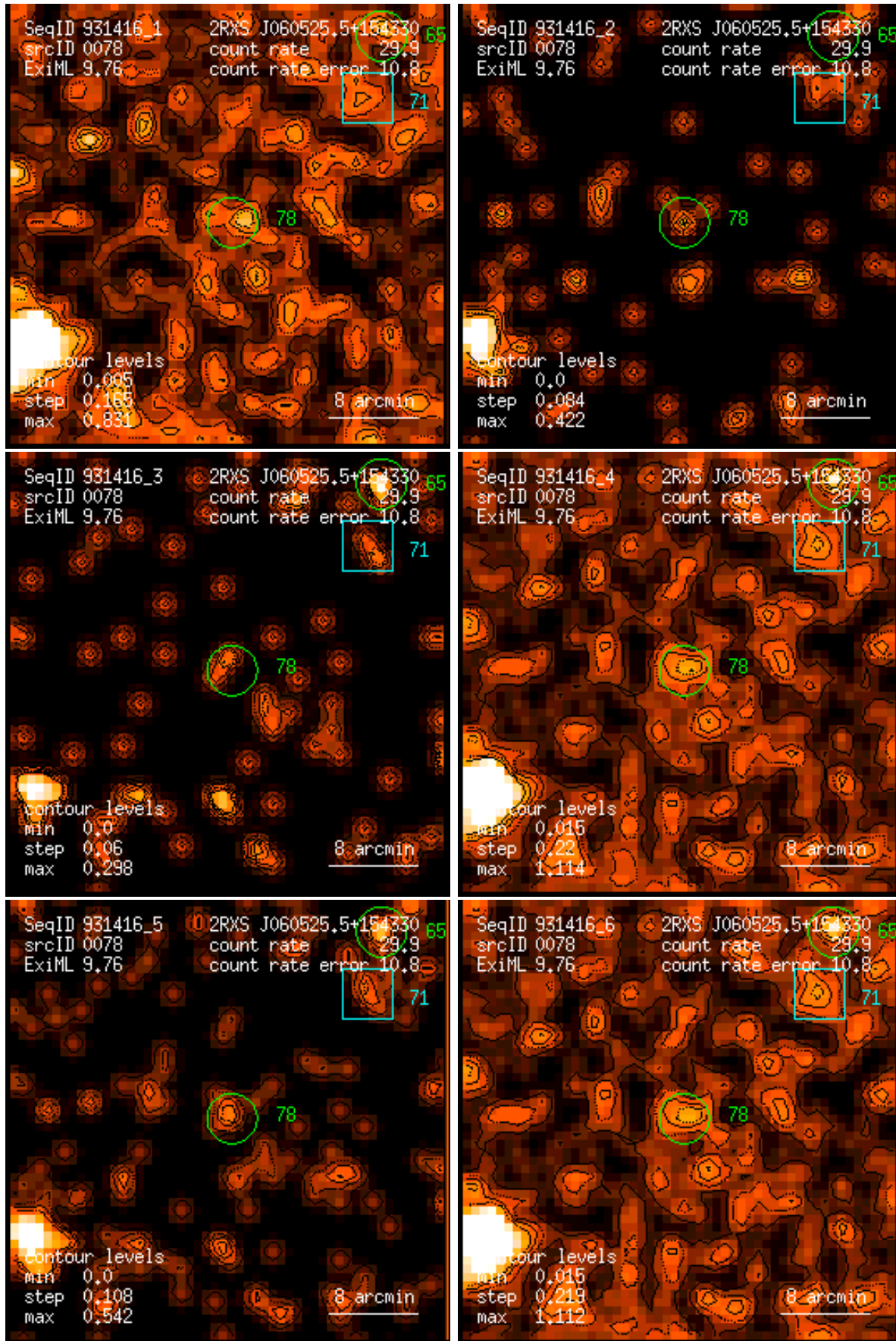
Figure 78: RASS 931416: detection 0078: band rate images, Gaussian filter: (1) PSPC channels 11 – 41, (2) 52 – 90, (3) 91 – 201, (4) 11 – 235, (5) 52 – 201, (6) 11 – 201. Broad band rates in counts/ks. Band rate contour levels in counts/ks/arcmin 2 .
