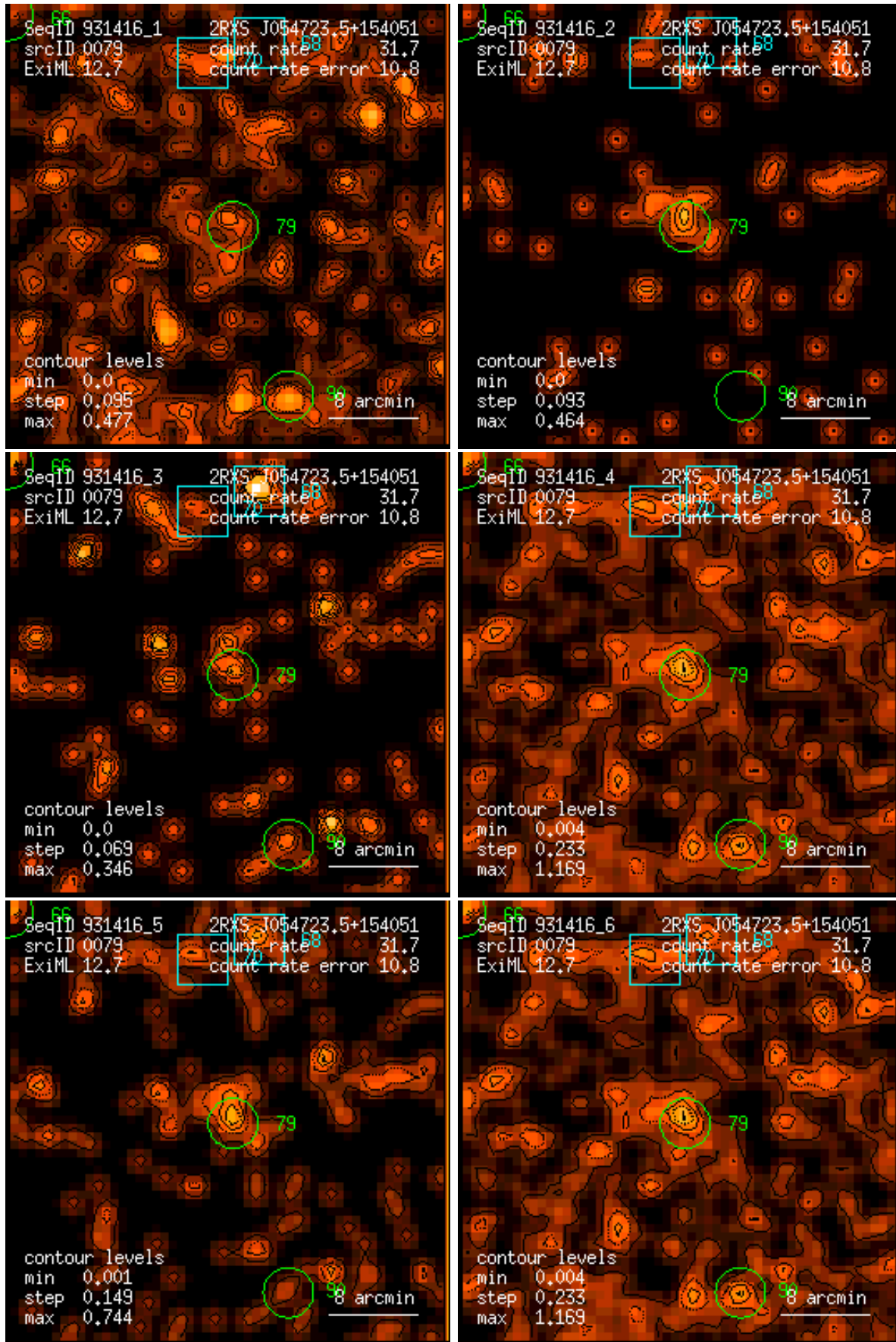
Figure 79: RASS 931416: detection 0079: band rate images, Gaussian filter: (1) PSPC channels 11 – 41, (2) 52 – 90, (3) 91 – 201, (4) 11 – 235, (5) 52 – 201, (6) 11 – 201. Broad band rates in counts/ks. Band rate contour levels in counts/ks/arcmin 2 .
