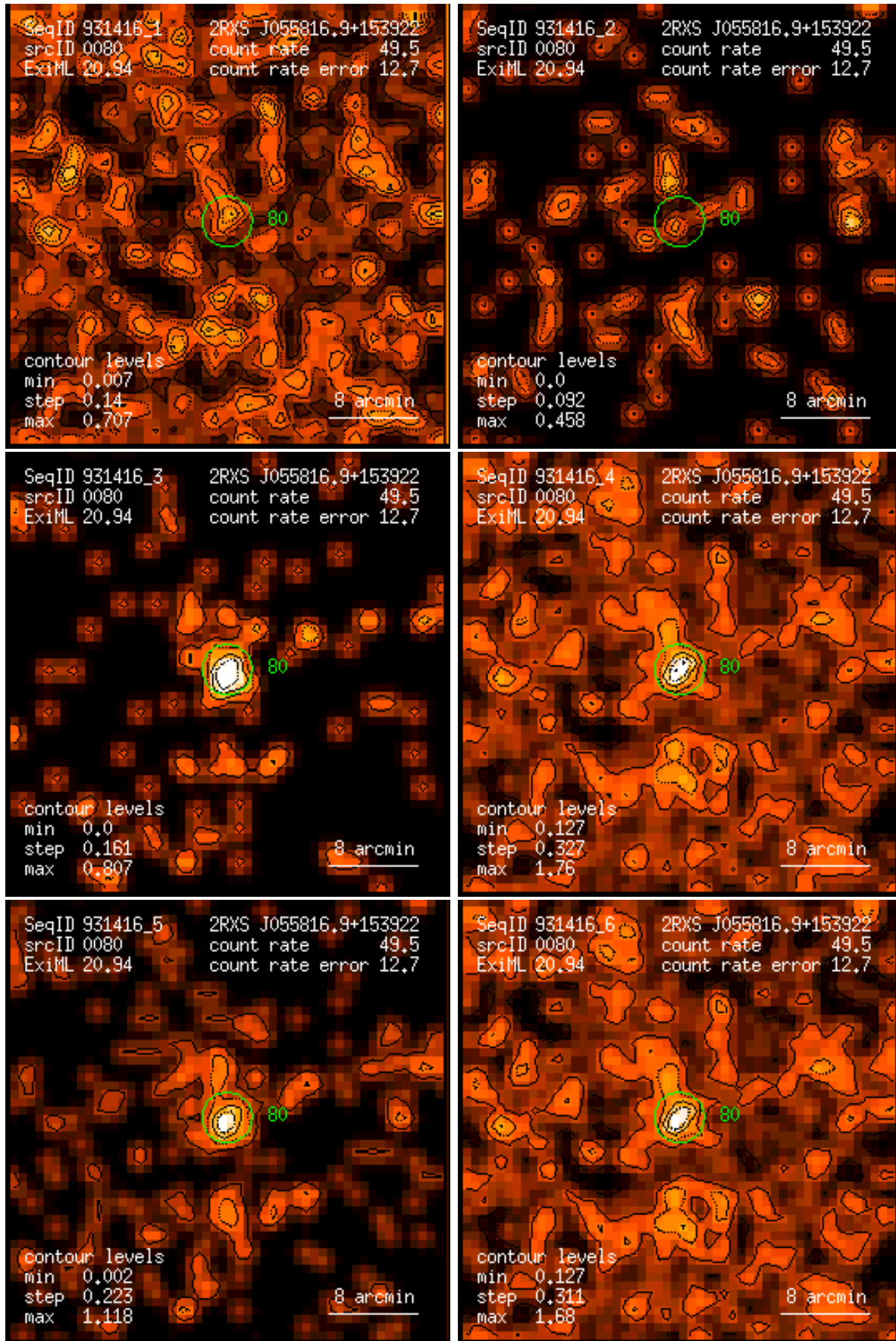
Figure 80: RASS 931416: detection 0080: band rate images, Gaussian filter: (1) PSPC channels 11 – 41, (2) 52 – 90, (3) 91 – 201, (4) 11 – 235, (5) 52 – 201, (6) 11 – 201. Broad band rates in counts/ks. Band rate contour levels in counts/ks/arcmin 2 .
