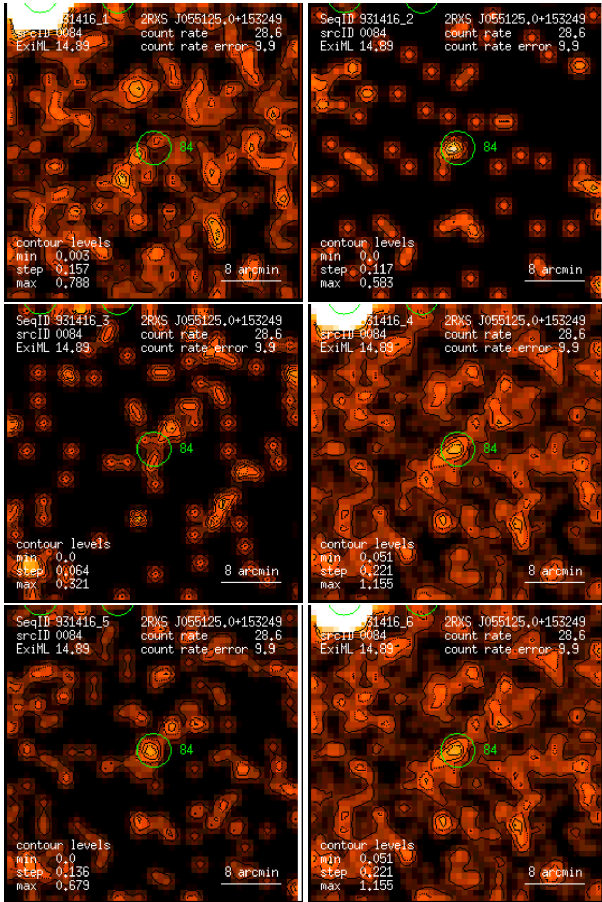
Figure 84: RASS 931416: detection 0084: band rate images, Gaussian filter: (1) PSPC channels 11 – 41, (2) 52 – 90, (3) 91 – 201, (4) 11 – 235, (5) 52 – 201, (6) 11 – 201. Broad band rates in counts/ks. Band rate contour levels in counts/ks/arcmin 2 .
