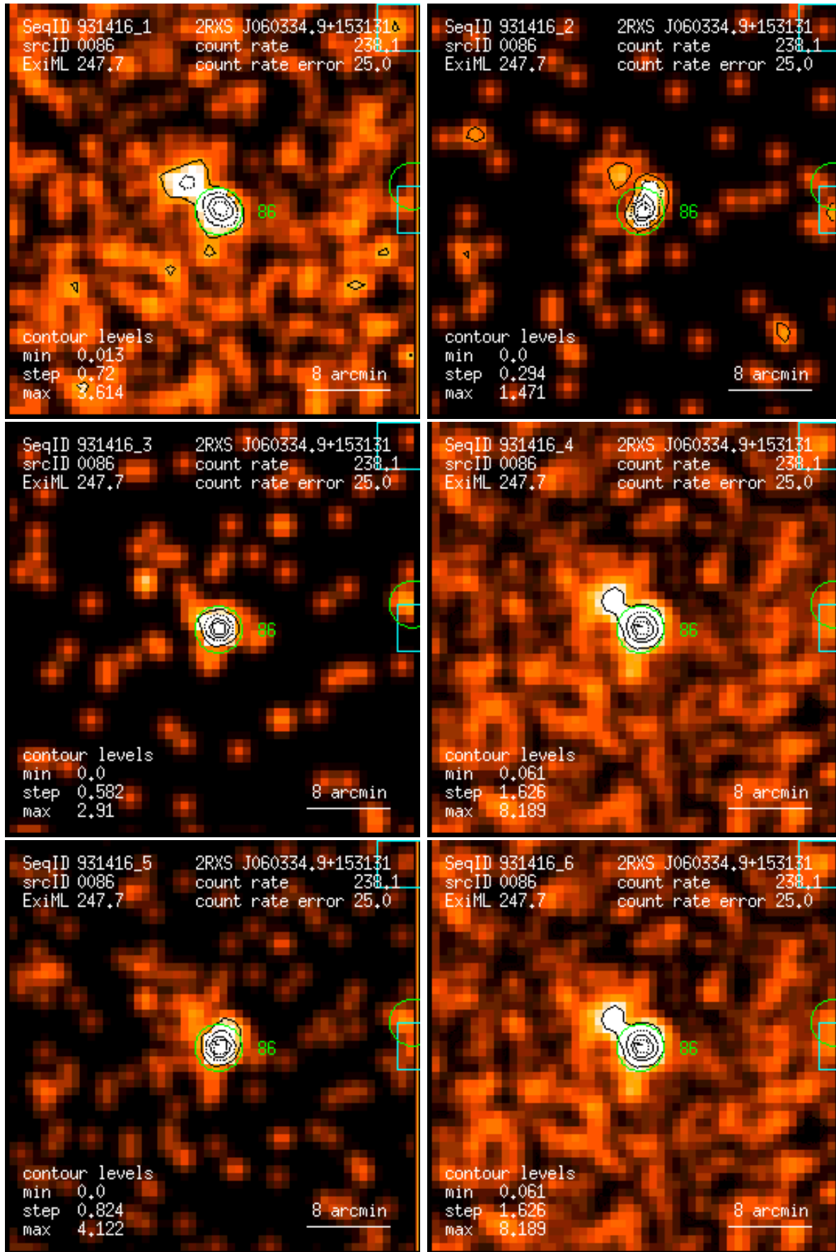
Figure 86: RASS 931416: detection 0086: band rate images, Gaussian filter: (1) PSPC channels 11 – 41, (2) 52 – 90, (3) 91 – 201, (4) 11 – 235, (5) 52 – 201, (6) 11 – 201. Broad band rates in counts/ks. Band rate contour levels in counts/ks/arcmin 2 .
