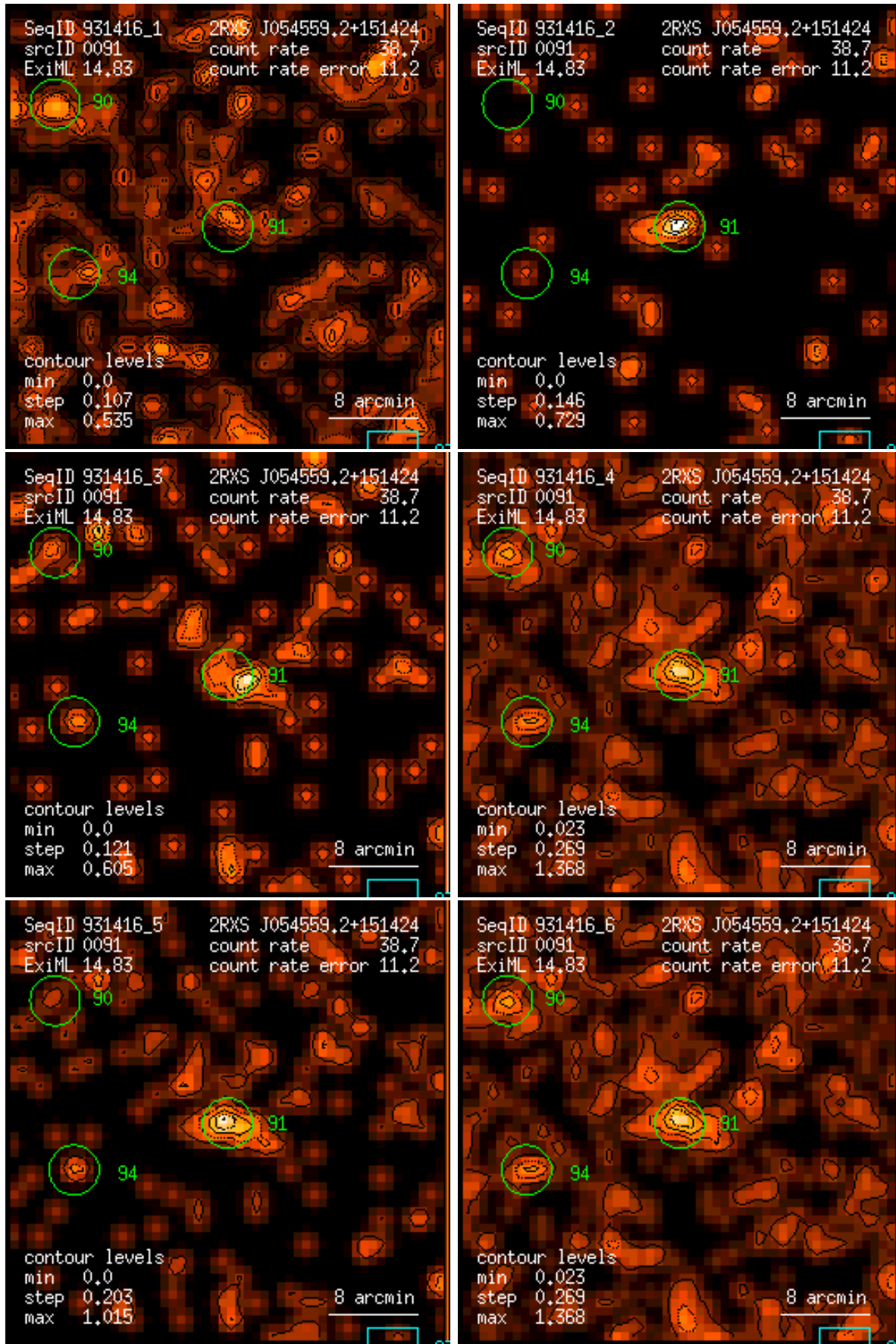
Figure 91: RASS 931416: detection 0091: band rate images, Gaussian filter: (1) PSPC channels 11 – 41, (2) 52 – 90, (3) 91 – 201, (4) 11 – 235, (5) 52 – 201, (6) 11 – 201. Broad band rates in counts/ks. Band rate contour levels in counts/ks/arcmin 2 .
