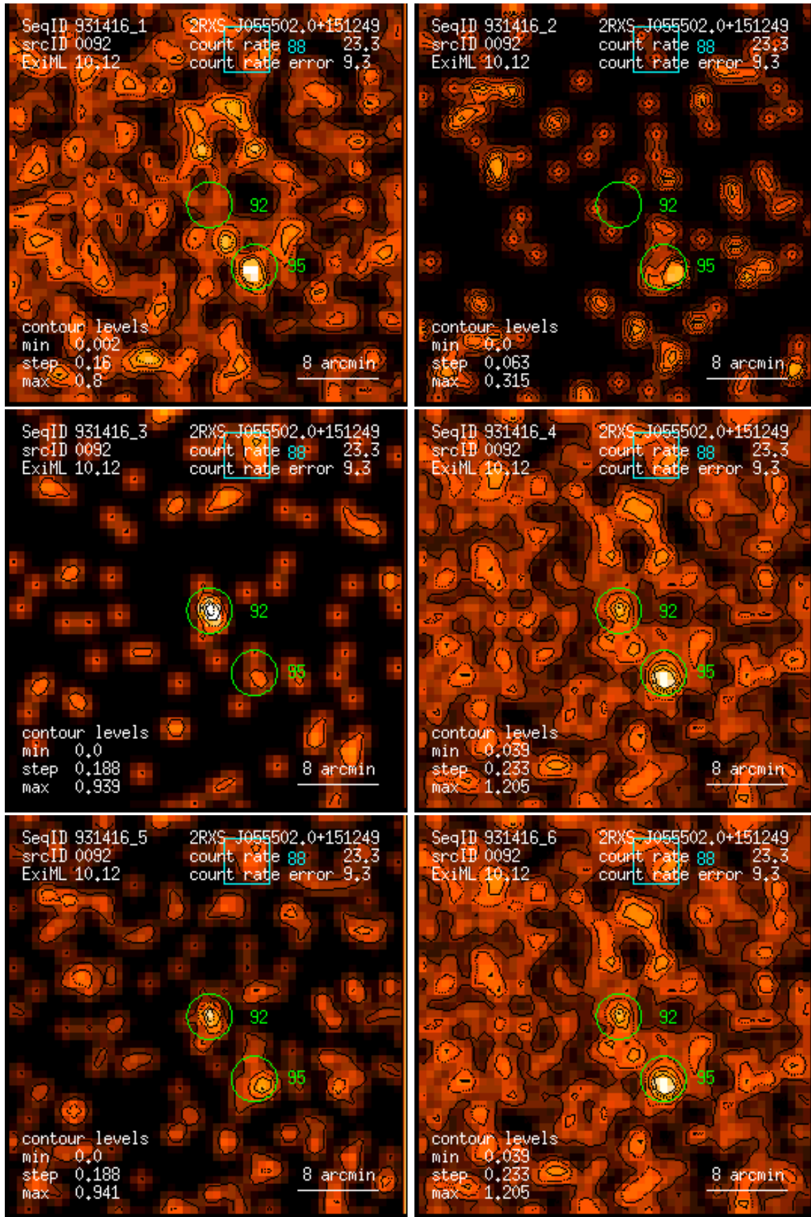
Figure 92: RASS 931416: detection 0092: band rate images, Gaussian filter: (1) PSPC channels 11 – 41, (2) 52 – 90, (3) 91 – 201, (4) 11 – 235, (5) 52 – 201, (6) 11 – 201. Broad band rates in counts/ks. Band rate contour levels in counts/ks/arcmin 2 .
