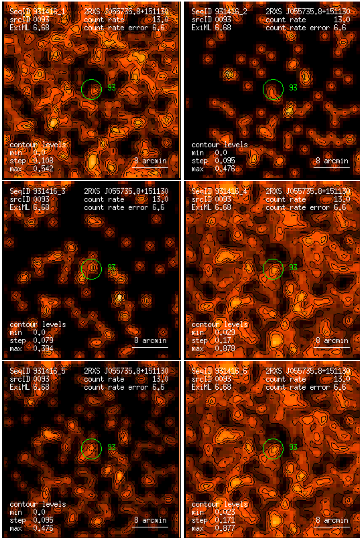
Figure 93: RASS 931416: detection 0093: band rate images, Gaussian filter: (1) PSPC channels 11 – 41, (2) 52 – 90, (3) 91 – 201, (4) 11 – 235, (5) 52 – 201, (6) 11 – 201. Broad band rates in counts/ks. Band rate contour levels in counts/ks/arcmin 2 .
