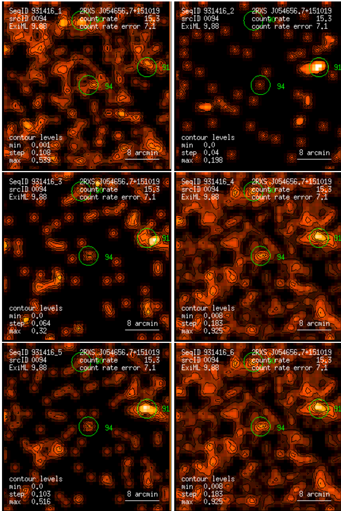
Figure 94: RASS 931416: detection 0094: band rate images, Gaussian filter: (1) PSPC channels 11 – 41, (2) 52 – 90, (3) 91 – 201, (4) 11 – 235, (5) 52 – 201, (6) 11 – 201. Broad band rates in counts/ks. Band rate contour levels in counts/ks/arcmin 2 .
