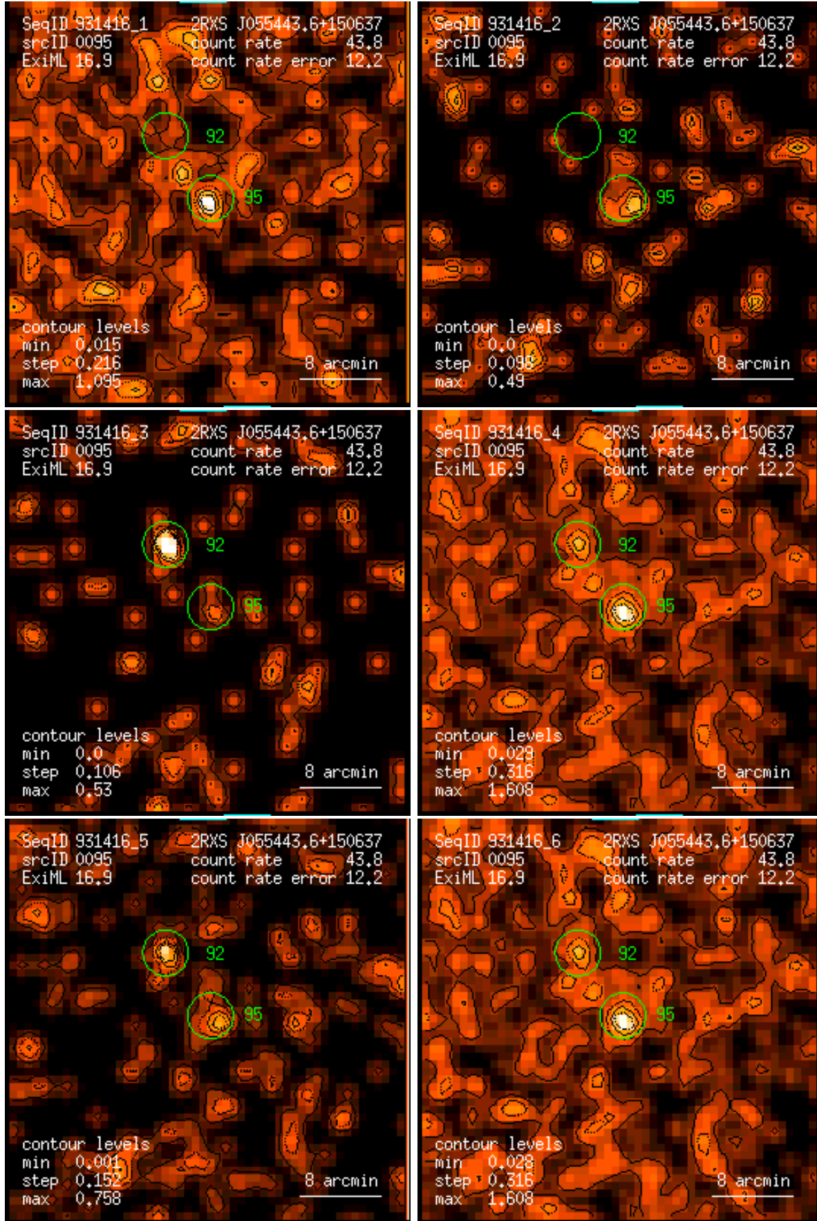
Figure 95: RASS 931416: detection 0095: band rate images, Gaussian filter: (1) PSPC channels 11 – 41, (2) 52 – 90, (3) 91 – 201, (4) 11 – 235, (5) 52 – 201, (6) 11 – 201. Broad band rates in counts/ks. Band rate contour levels in counts/ks/arcmin 2 .
