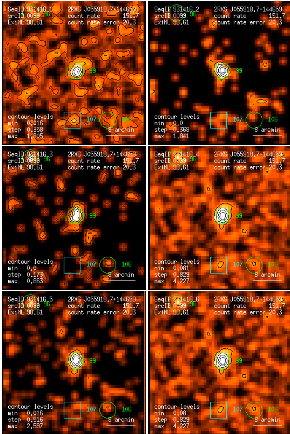
Figure 99: RASS 931416: detection 0099: band rate images, Gaussian filter: (1) PSPC channels 11 – 41, (2) 52 – 90, (3) 91 – 201, (4) 11 – 235, (5) 52 – 201, (6) 11 – 201. Broad band rates in counts/ks. Band rate contour levels in counts/ks/arcmin 2 .
