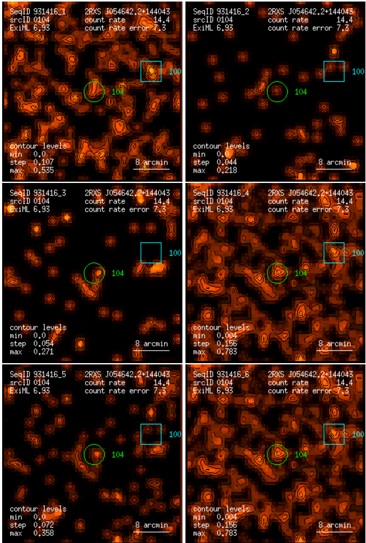
Figure 104: RASS 931416: detection 0104: band rate images, Gaussian filter: (1) PSPC channels 11 – 41, (2) 52 – 90, (3) 91 – 201, (4) 11 – 235, (5) 52 – 201, (6) 11 – 201. Broad band rates in counts/ks. Band rate contour levels in counts/ks/arcmin 2 .
