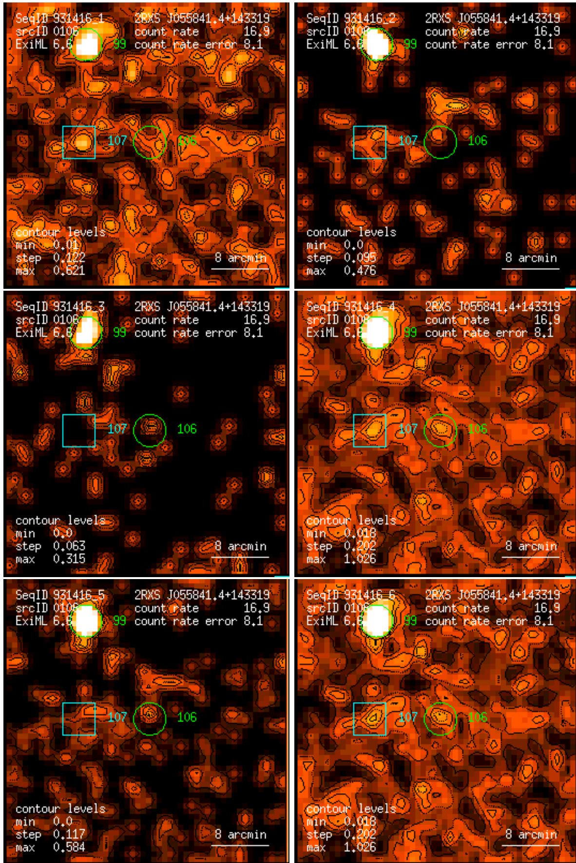
Figure 106: RASS 931416: detection 0106: band rate images, Gaussian filter: (1) PSPC channels 11 – 41, (2) 52 – 90, (3) 91 – 201, (4) 11 – 235, (5) 52 – 201, (6) 11 – 201. Broad band rates in counts/ks. Band rate contour levels in counts/ks/arcmin 2 .
