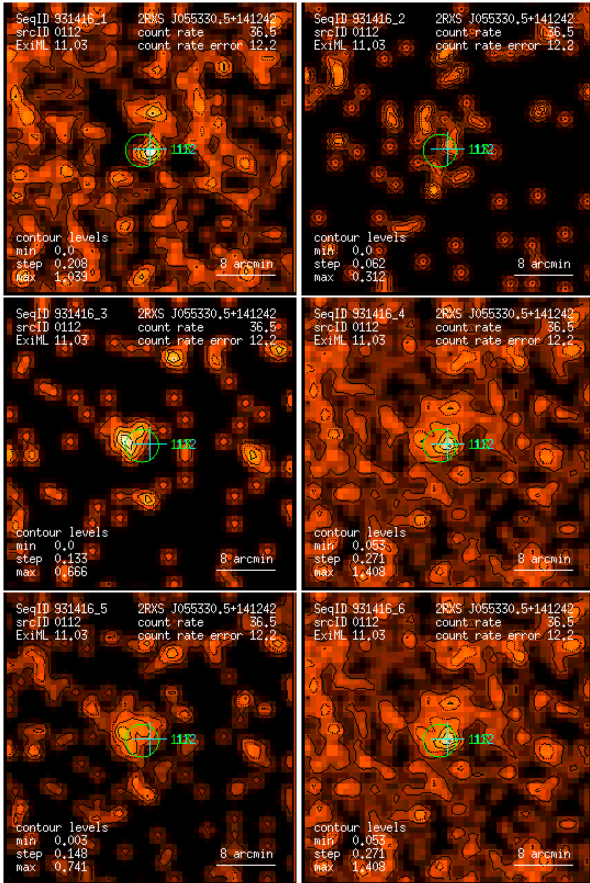
Figure 112: RASS 931416: detection 0112: band rate images, Gaussian filter: (1) PSPC channels 11 – 41, (2) 52 – 90, (3) 91 – 201, (4) 11 – 235, (5) 52 – 201, (6) 11 – 201. Broad band rates in counts/ks. Band rate contour levels in counts/ks/arcmin 2 .
