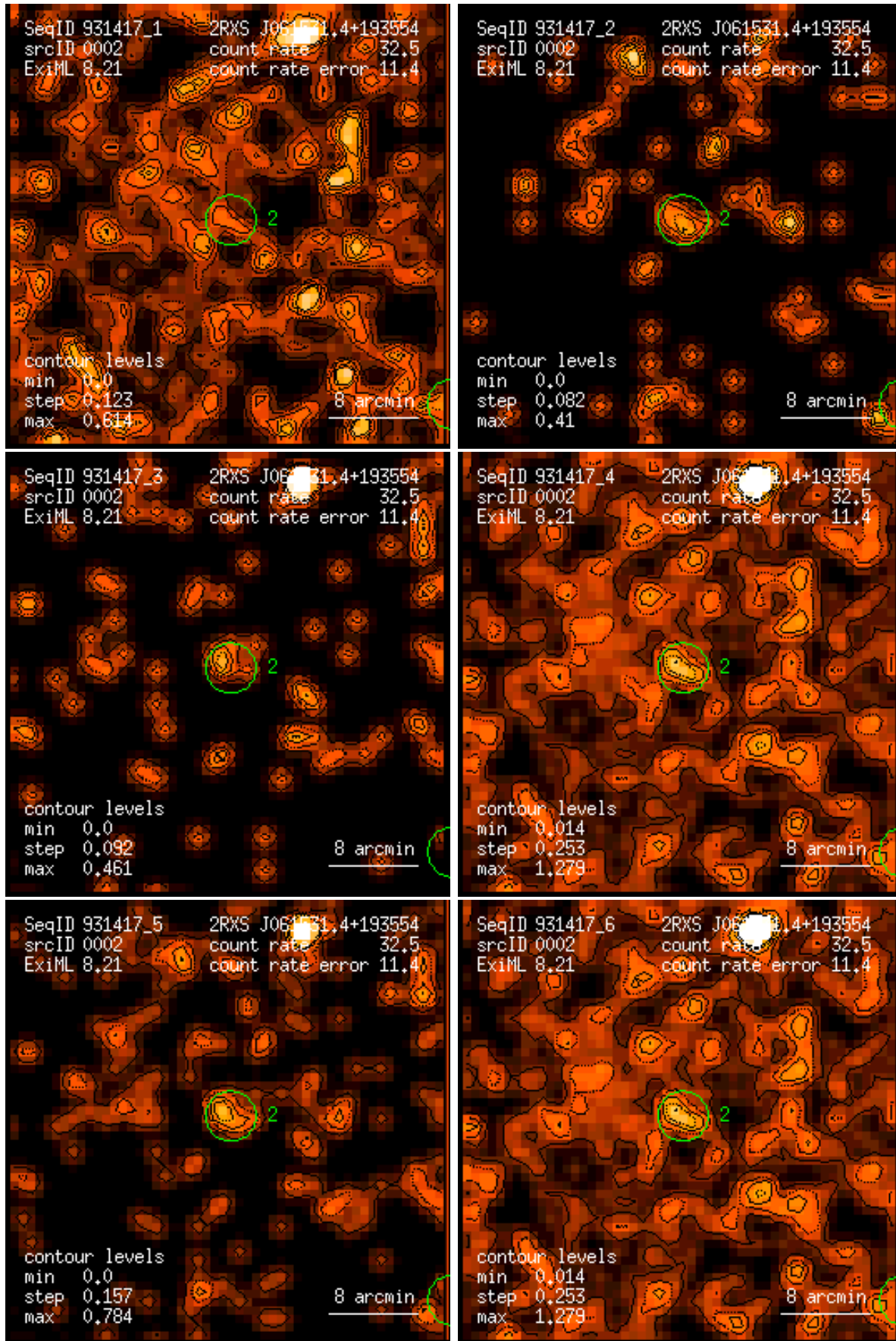
Figure 2: RASS 931417: detection 0002: band rate images, Gaussian filter: (1) PSPC channels 11 – 41, (2) 52 – 90, (3) 91 – 201, (4) 11 – 235, (5) 52 – 201, (6) 11 – 201. Broad band rates in counts/ks. Band rate contour levels in counts/ks/arcmin 2 .
