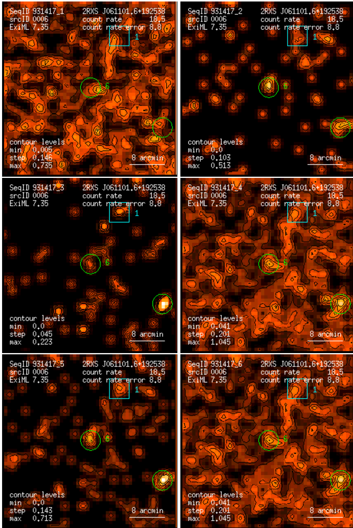
Figure 6: RASS 931417: detection 0006: band rate images, Gaussian filter: (1) PSPC channels 11 – 41, (2) 52 – 90, (3) 91 – 201, (4) 11 – 235, (5) 52 – 201, (6) 11 – 201. Broad band rates in counts/ks. Band rate contour levels in counts/ks/arcmin 2 .
