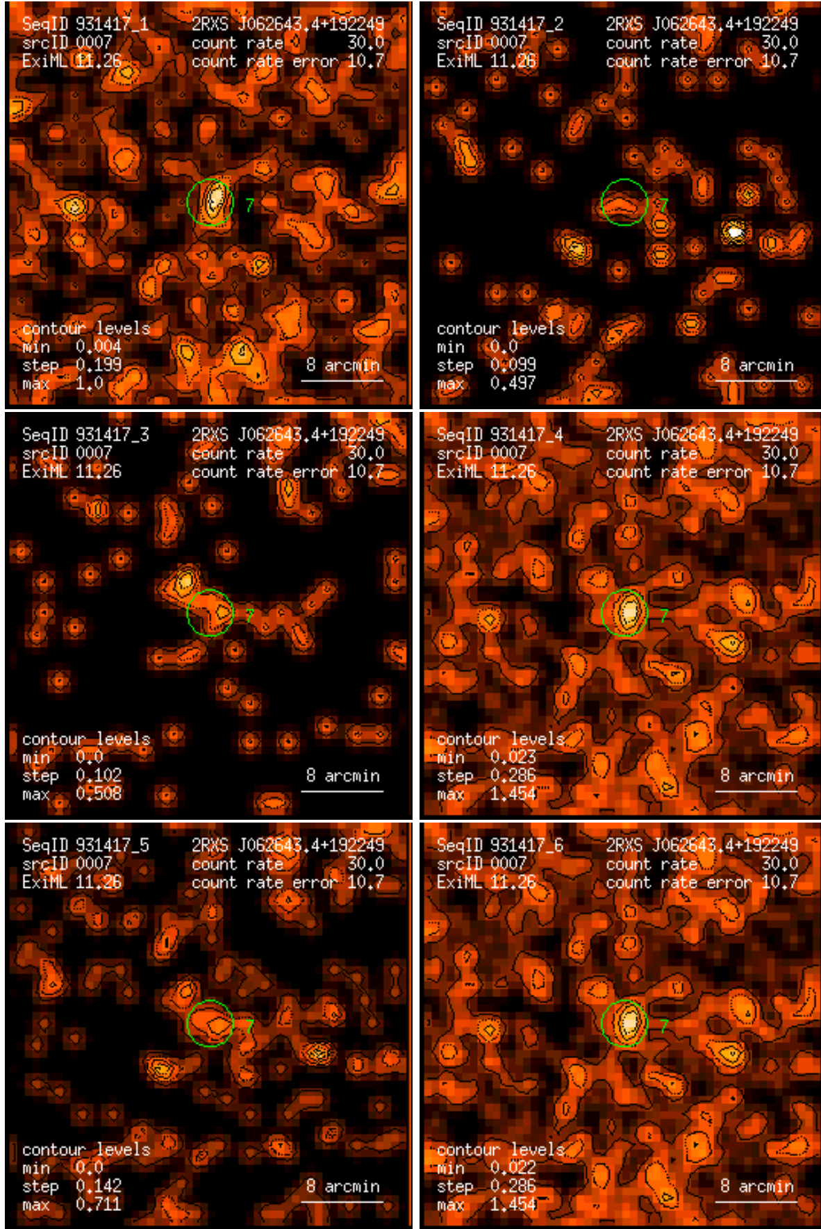
Figure 7: RASS 931417: detection 0007: band rate images, Gaussian filter: (1) PSPC channels 11 – 41, (2) 52 – 90, (3) 91 – 201, (4) 11 – 235, (5) 52 – 201, (6) 11 – 201. Broad band rates in counts/ks. Band rate contour levels in counts/ks/arcmin 2 .
