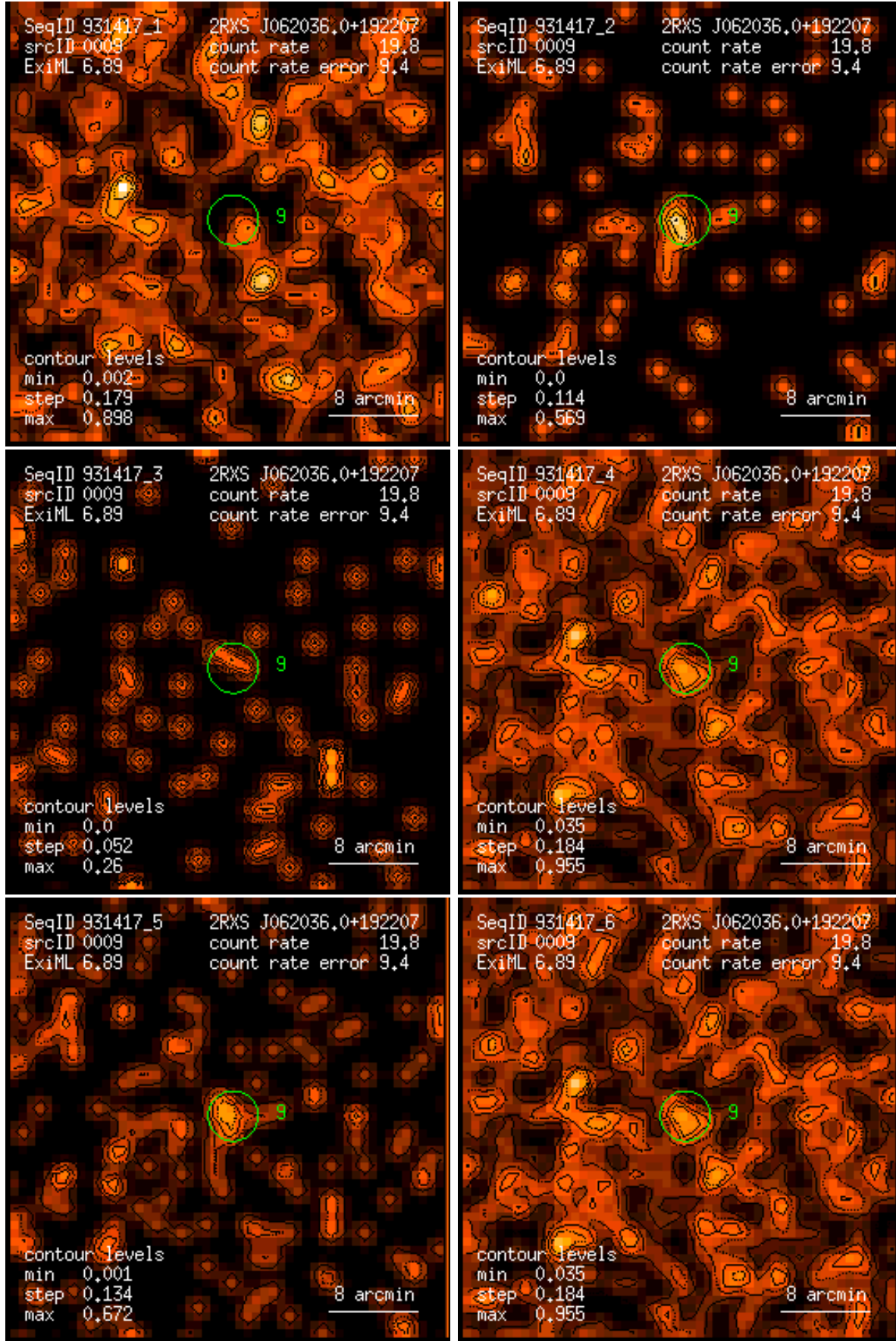
Figure 9: RASS 931417: detection 0009: band rate images, Gaussian filter: (1) PSPC channels 11 – 41, (2) 52 – 90, (3) 91 – 201, (4) 11 – 235, (5) 52 – 201, (6) 11 – 201. Broad band rates in counts/ks. Band rate contour levels in counts/ks/arcmin 2 .
