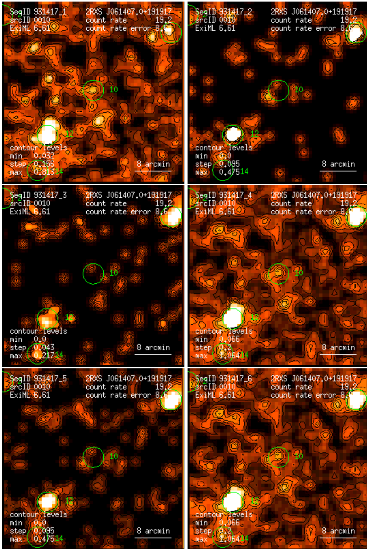
Figure 10: RASS 931417: detection 0010: band rate images, Gaussian filter: (1) PSPC channels 11 – 41, (2) 52 – 90, (3) 91 – 201, (4) 11 – 235, (5) 52 – 201, (6) 11 – 201. Broad band rates in counts/ks. Band rate contour levels in counts/ks/arcmin 2 .
