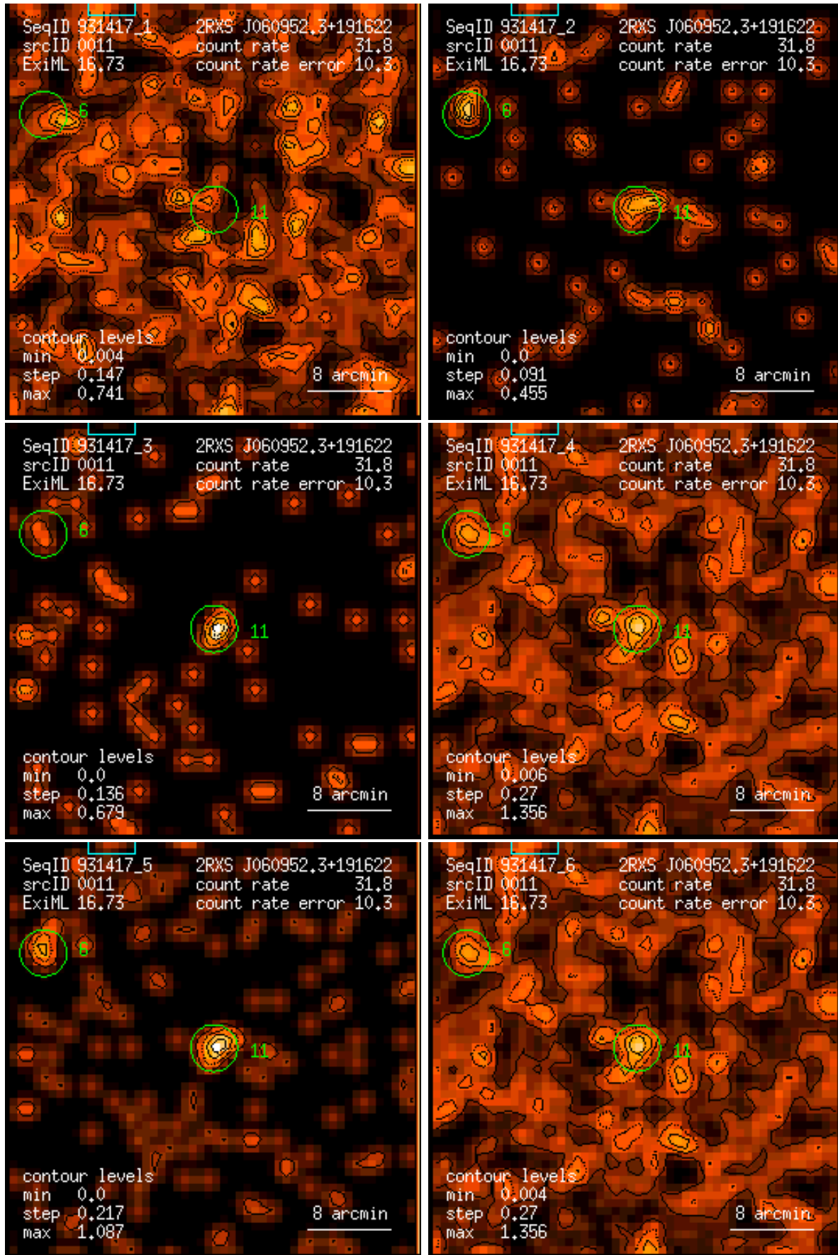
Figure 11: RASS 931417: detection 0011: band rate images, Gaussian filter: (1) PSPC channels 11 – 41, (2) 52 – 90, (3) 91 – 201, (4) 11 – 235, (5) 52 – 201, (6) 11 – 201. Broad band rates in counts/ks. Band rate contour levels in counts/ks/arcmin 2 .
