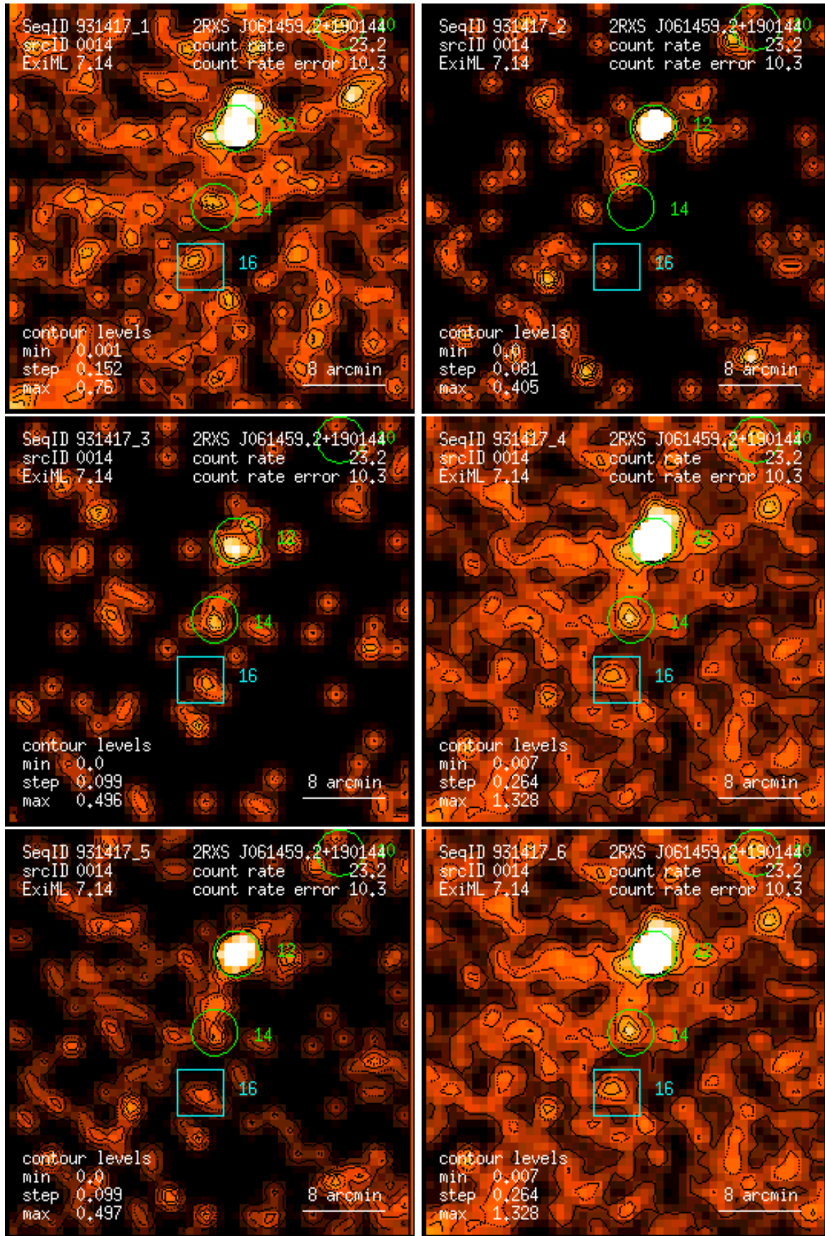
Figure 14: RASS 931417: detection 0014: band rate images, Gaussian filter: (1) PSPC channels 11 – 41, (2) 52 – 90, (3) 91 – 201, (4) 11 – 235, (5) 52 – 201, (6) 11 – 201. Broad band rates in counts/ks. Band rate contour levels in counts/ks/arcmin 2 .
