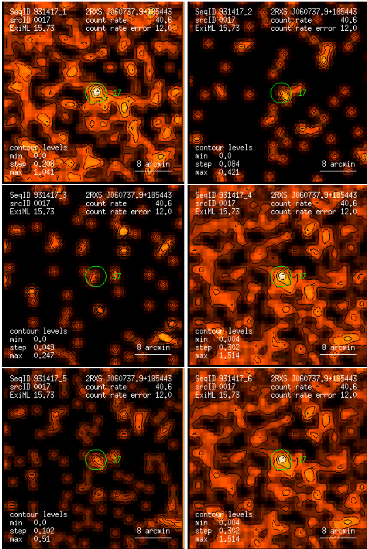
Figure 17: RASS 931417: detection 0017: band rate images, Gaussian filter: (1) PSPC channels 11 – 41, (2) 52 – 90, (3) 91 – 201, (4) 11 – 235, (5) 52 – 201, (6) 11 – 201. Broad band rates in counts/ks. Band rate contour levels in counts/ks/arcmin 2 .
