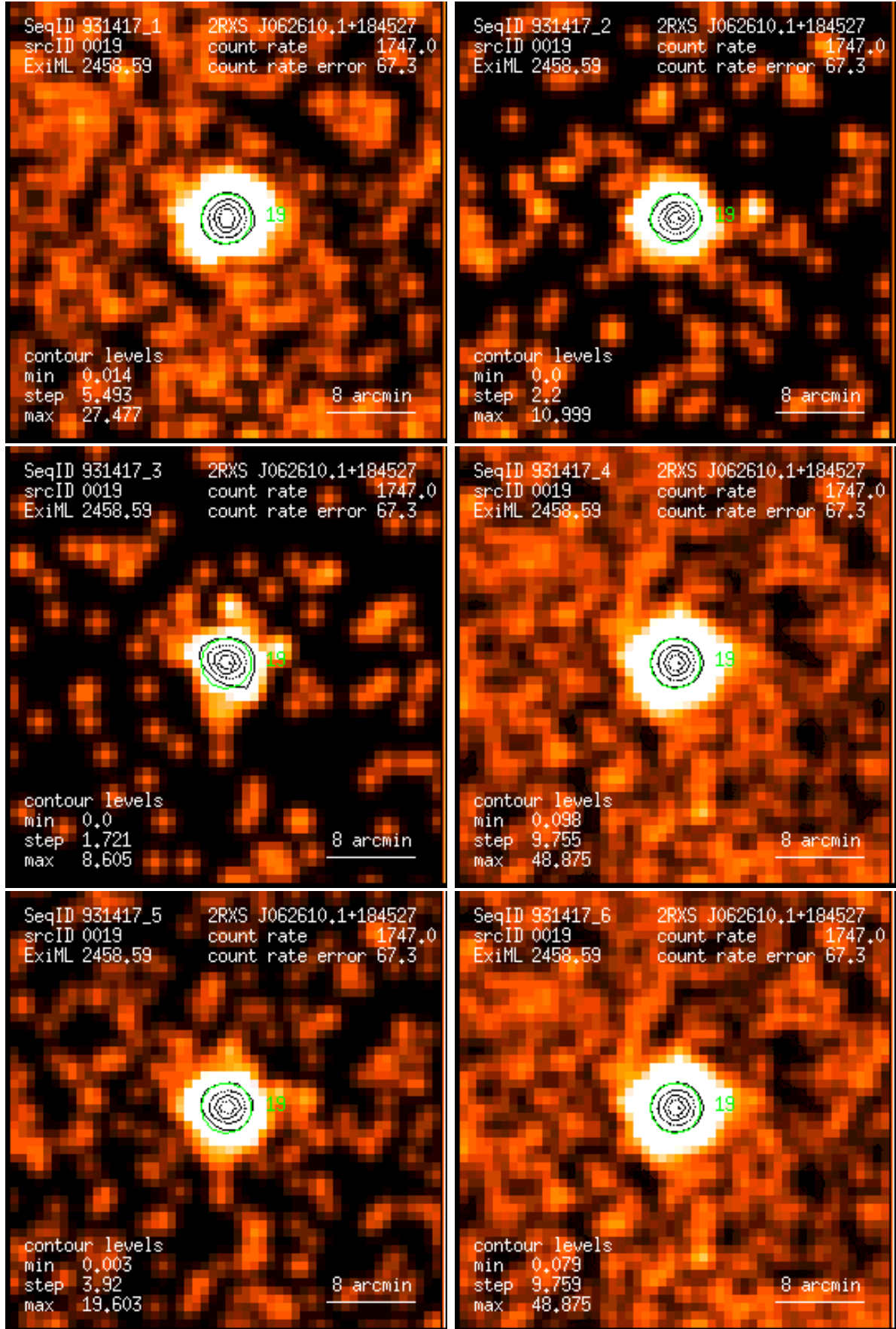
Figure 19: RASS 931417: detection 0019: band rate images, Gaussian filter: (1) PSPC channels 11 – 41, (2) 52 – 90, (3) 91 – 201, (4) 11 – 235, (5) 52 – 201, (6) 11 – 201. Broad band rates in counts/ks. Band rate contour levels in counts/ks/arcmin 2 .
