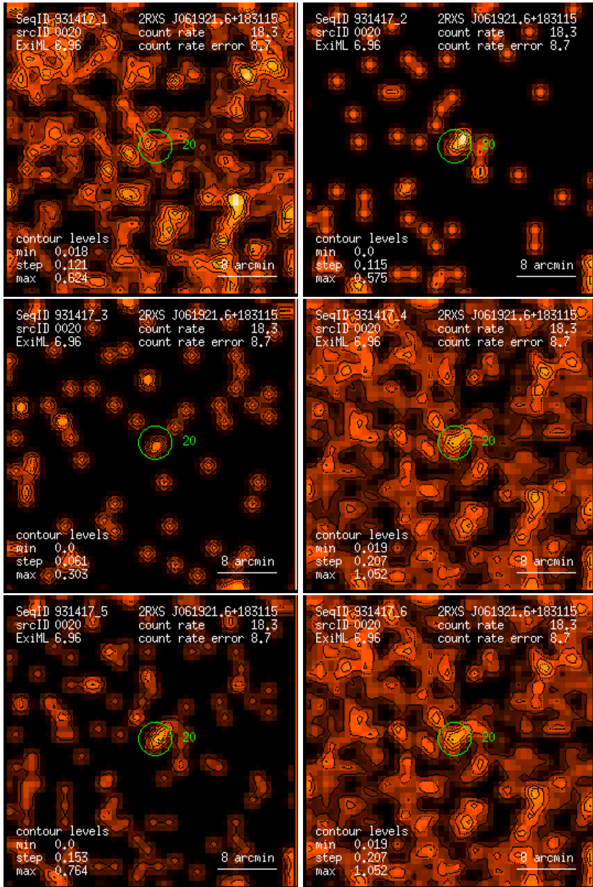
Figure 20: RASS 931417: detection 0020: band rate images, Gaussian filter: (1) PSPC channels 11 – 41, (2) 52 – 90, (3) 91 – 201, (4) 11 – 235, (5) 52 – 201, (6) 11 – 201. Broad band rates in counts/ks. Band rate contour levels in counts/ks/arcmin 2 .
