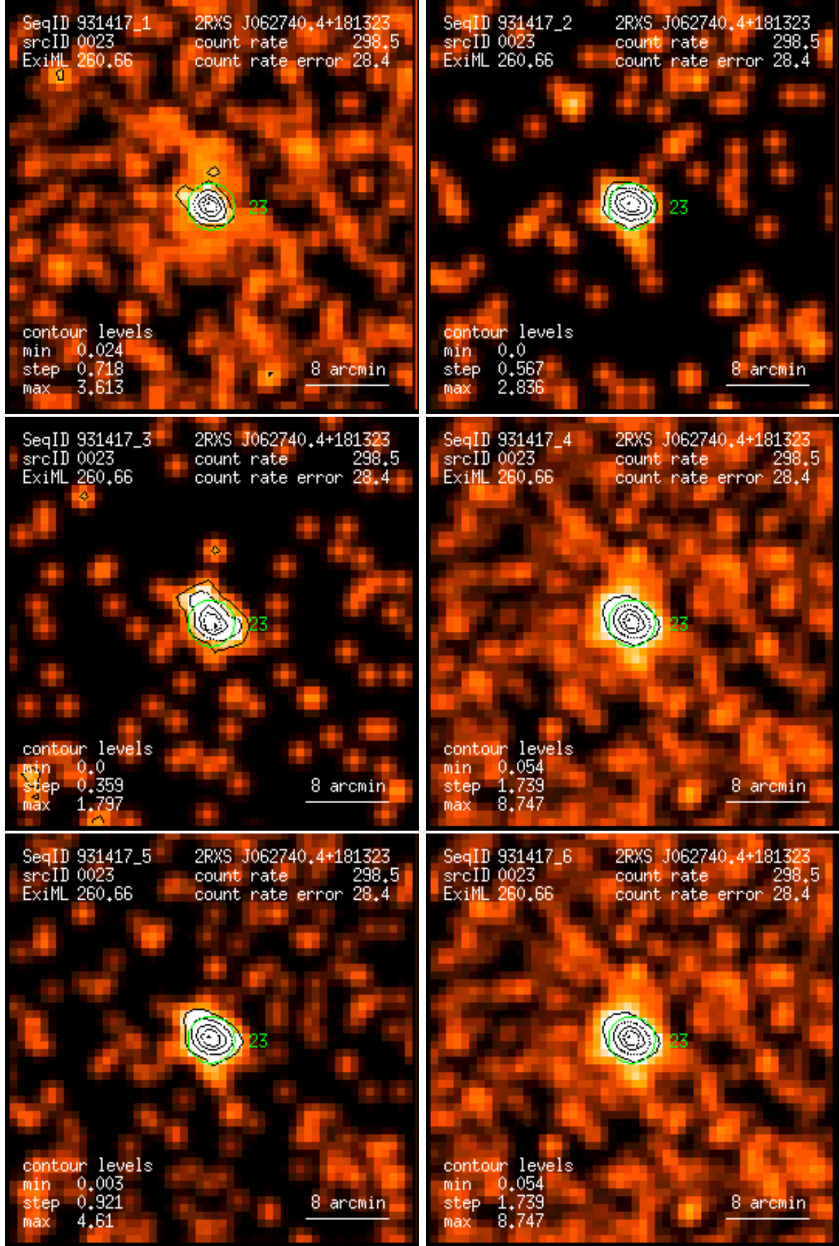
Figure 23: RASS 931417: detection 0023: band rate images, Gaussian filter: (1) PSPC channels 11 – 41, (2) 52 – 90, (3) 91 – 201, (4) 11 – 235, (5) 52 – 201, (6) 11 – 201. Broad band rates in counts/ks. Band rate contour levels in counts/ks/arcmin 2 .
