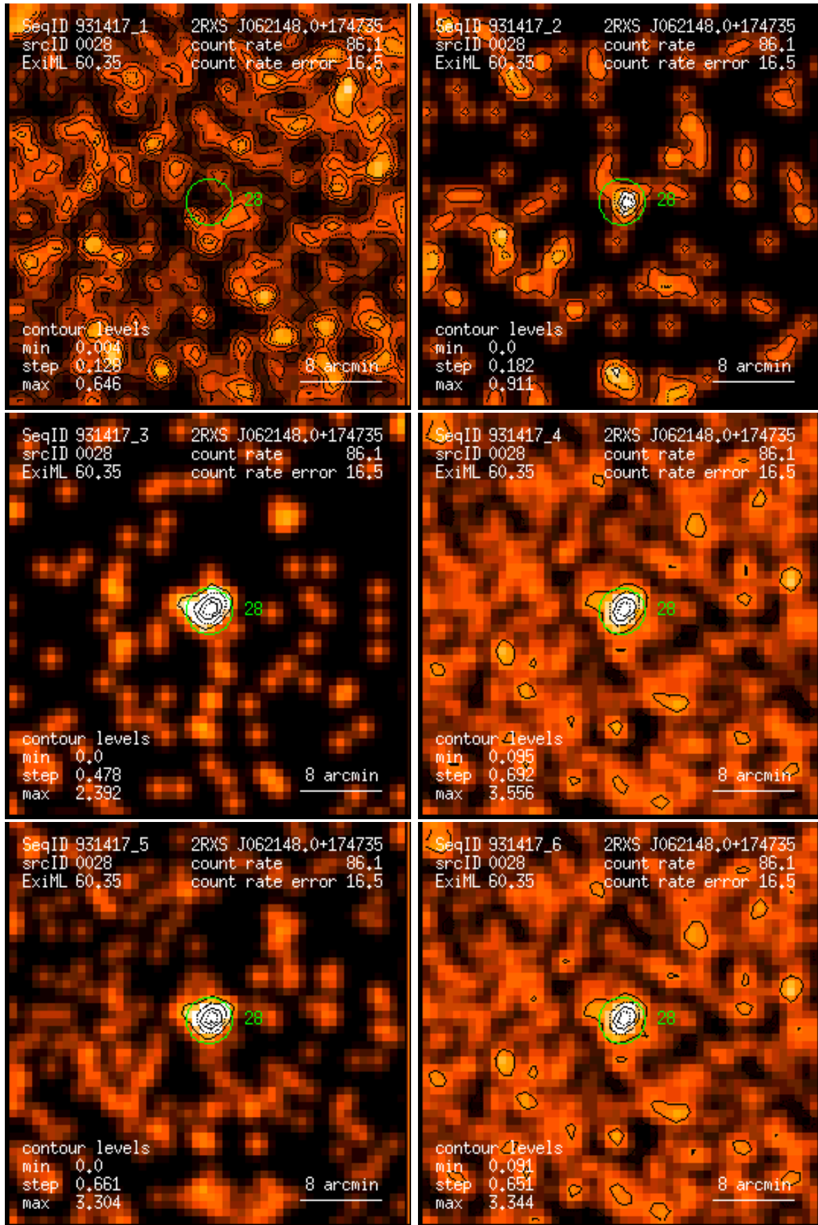
Figure 28: RASS 931417: detection 0028: band rate images, Gaussian filter: (1) PSPC channels 11 – 41, (2) 52 – 90, (3) 91 – 201, (4) 11 – 235, (5) 52 – 201, (6) 11 – 201. Broad band rates in counts/ks. Band rate contour levels in counts/ks/arcmin 2 .
