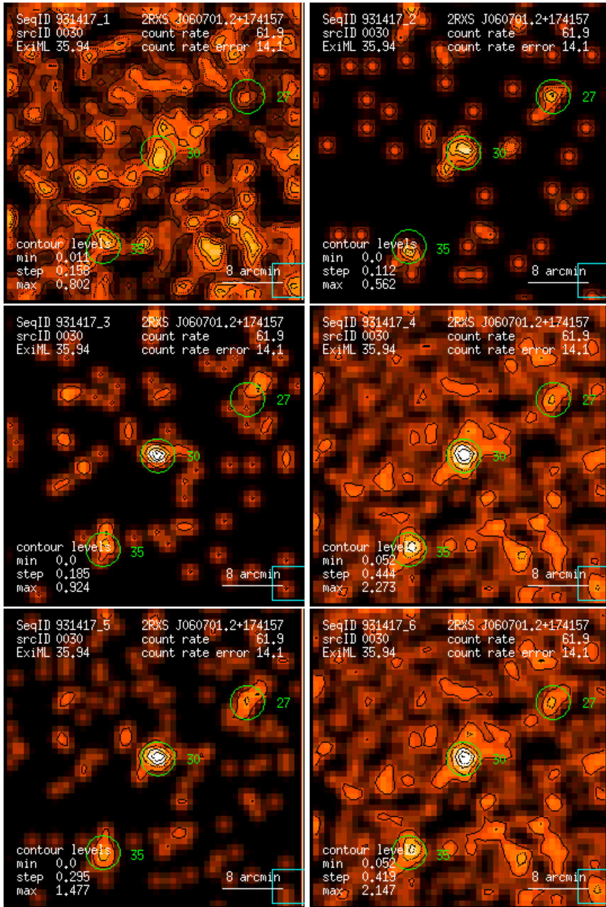
Figure 30: RASS 931417: detection 0030: band rate images, Gaussian filter: (1) PSPC channels 11 – 41, (2) 52 – 90, (3) 91 – 201, (4) 11 – 235, (5) 52 – 201, (6) 11 – 201. Broad band rates in counts/ks. Band rate contour levels in counts/ks/arcmin 2 .
