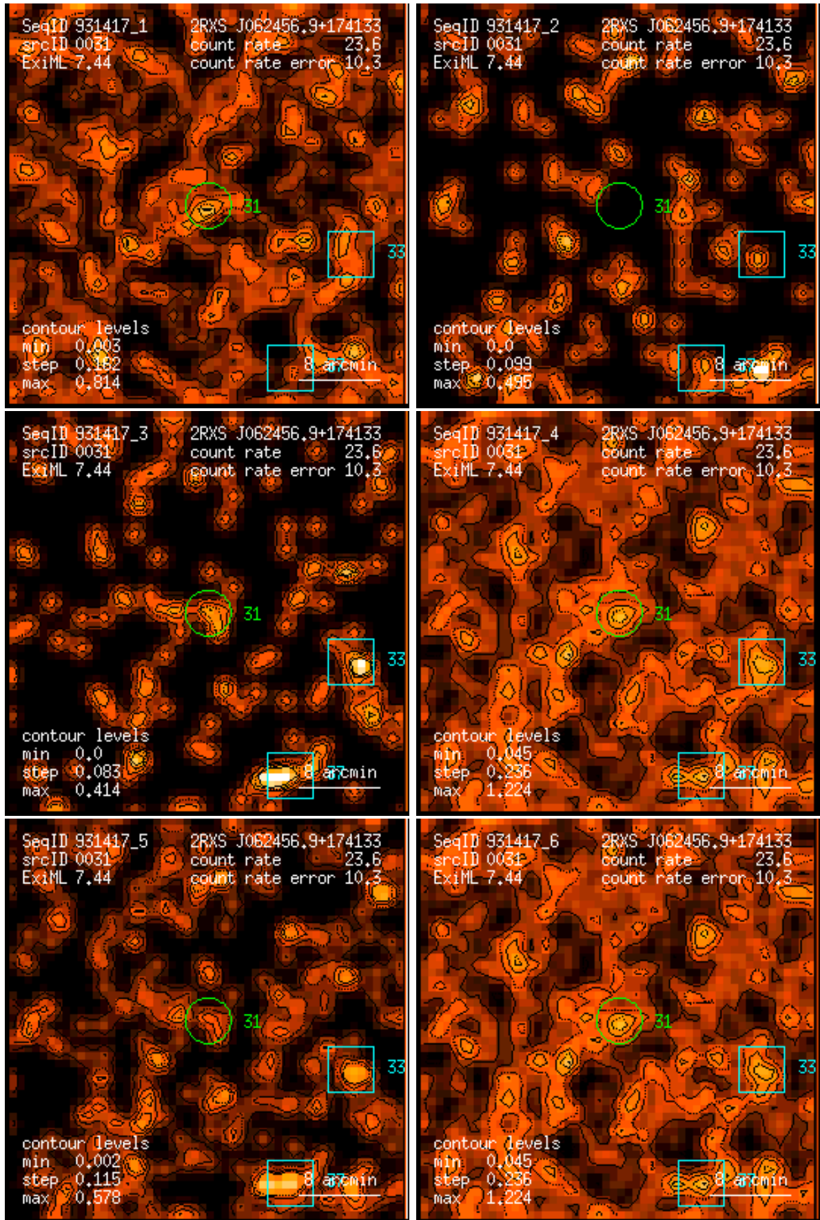
Figure 31: RASS 931417: detection 0031: band rate images, Gaussian filter: (1) PSPC channels 11 – 41, (2) 52 – 90, (3) 91 – 201, (4) 11 – 235, (5) 52 – 201, (6) 11 – 201. Broad band rates in counts/ks. Band rate contour levels in counts/ks/arcmin 2 .
