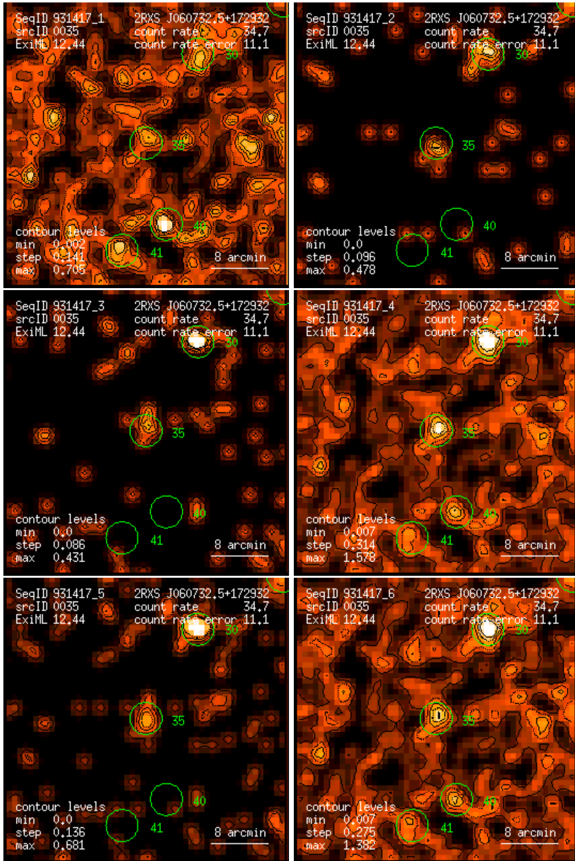
Figure 35: RASS 931417: detection 0035: band rate images, Gaussian filter: (1) PSPC channels 11 – 41, (2) 52 – 90, (3) 91 – 201, (4) 11 – 235, (5) 52 – 201, (6) 11 – 201. Broad band rates in counts/ks. Band rate contour levels in counts/ks/arcmin 2 .
