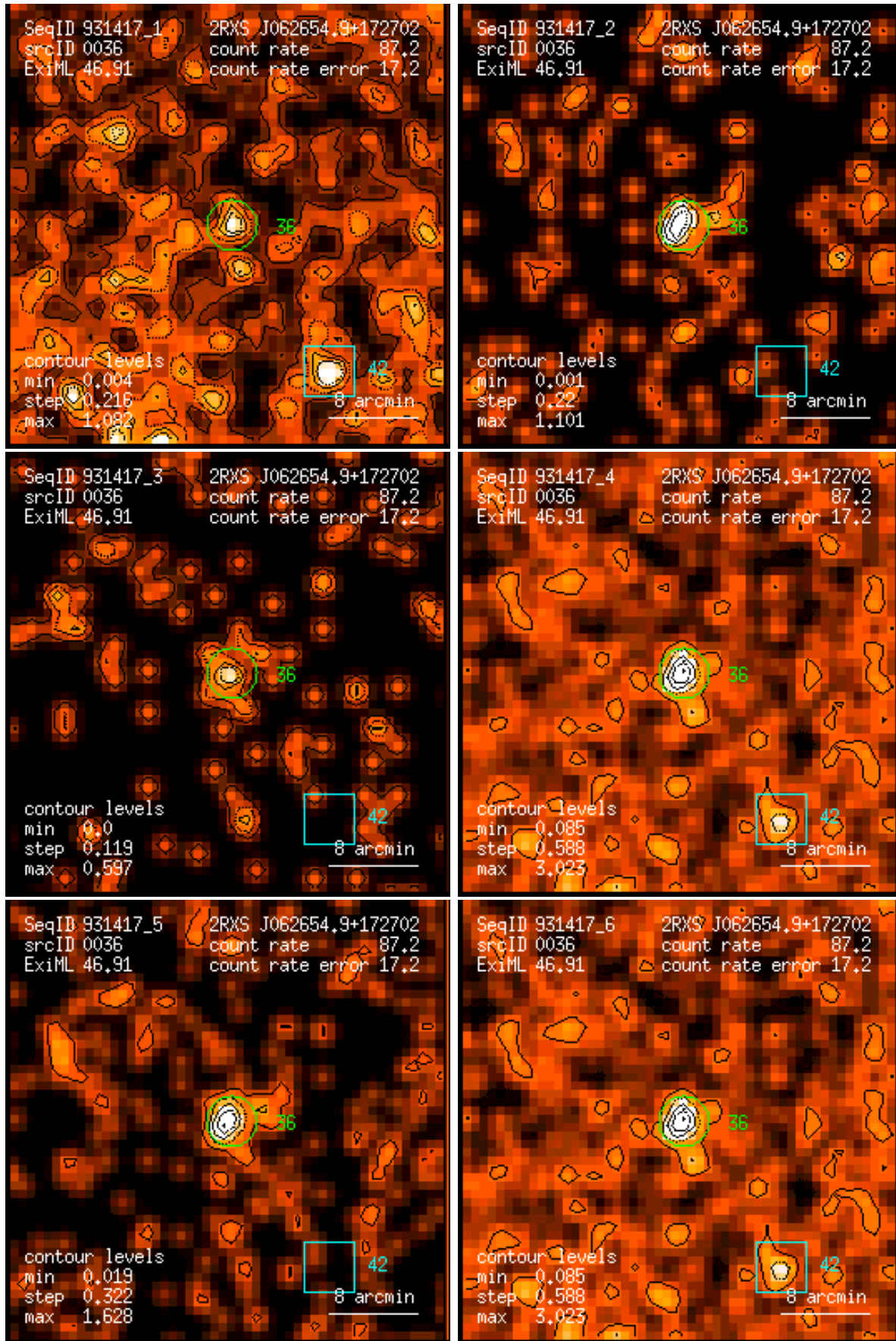
Figure 36: RASS 931417: detection 0036: band rate images, Gaussian filter: (1) PSPC channels 11 – 41, (2) 52 – 90, (3) 91 – 201, (4) 11 – 235, (5) 52 – 201, (6) 11 – 201. Broad band rates in counts/ks. Band rate contour levels in counts/ks/arcmin 2 .
