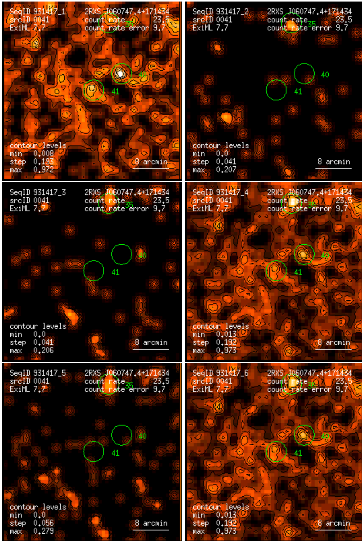
Figure 41: RASS 931417: detection 0041: band rate images, Gaussian filter: (1) PSPC channels 11 – 41, (2) 52 – 90, (3) 91 – 201, (4) 11 – 235, (5) 52 – 201, (6) 11 – 201. Broad band rates in counts/ks. Band rate contour levels in counts/ks/arcmin 2 .
