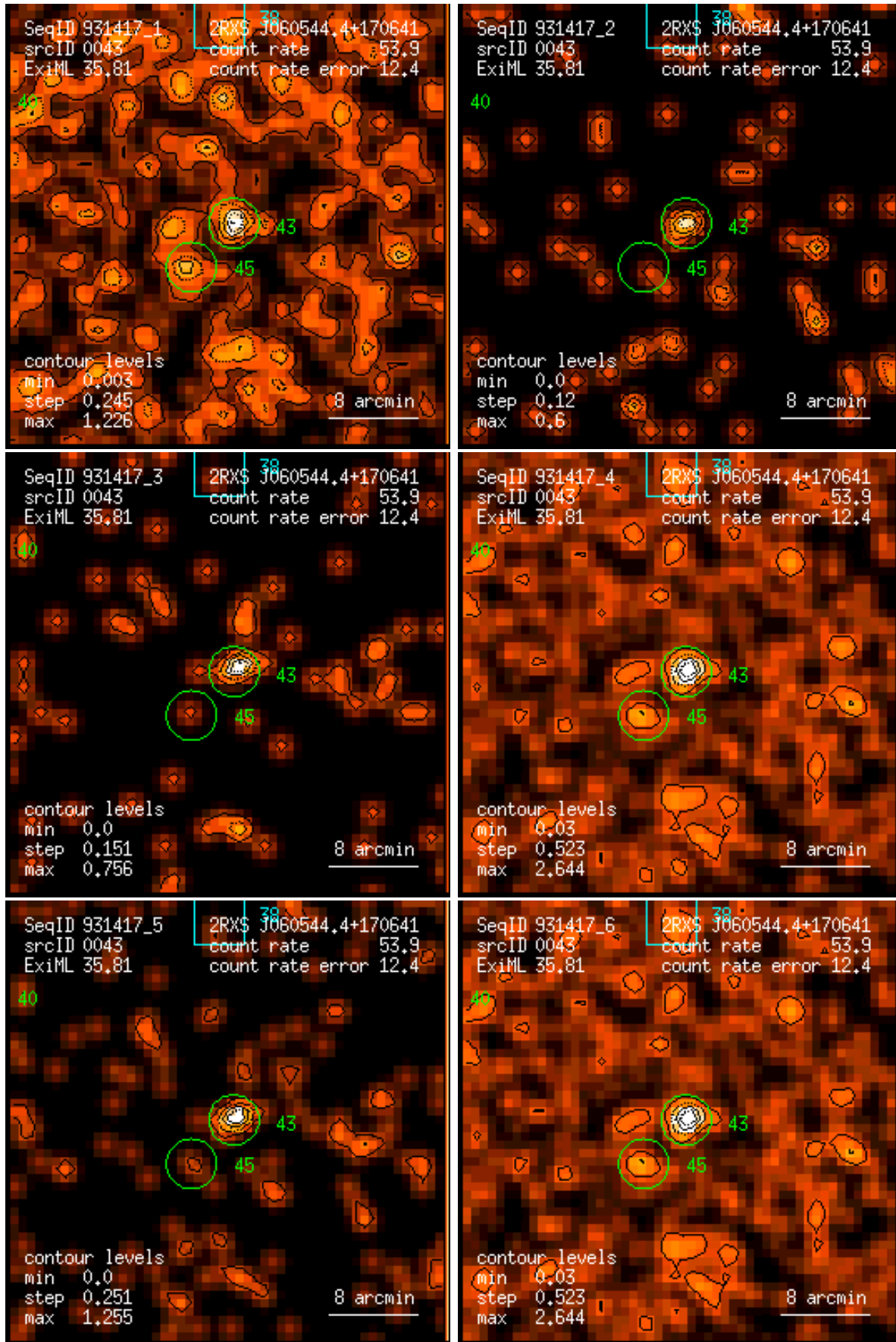
Figure 43: RASS 931417: detection 0043: band rate images, Gaussian filter: (1) PSPC channels 11 – 41, (2) 52 – 90, (3) 91 – 201, (4) 11 – 235, (5) 52 – 201, (6) 11 – 201. Broad band rates in counts/ks. Band rate contour levels in counts/ks/arcmin 2 .
