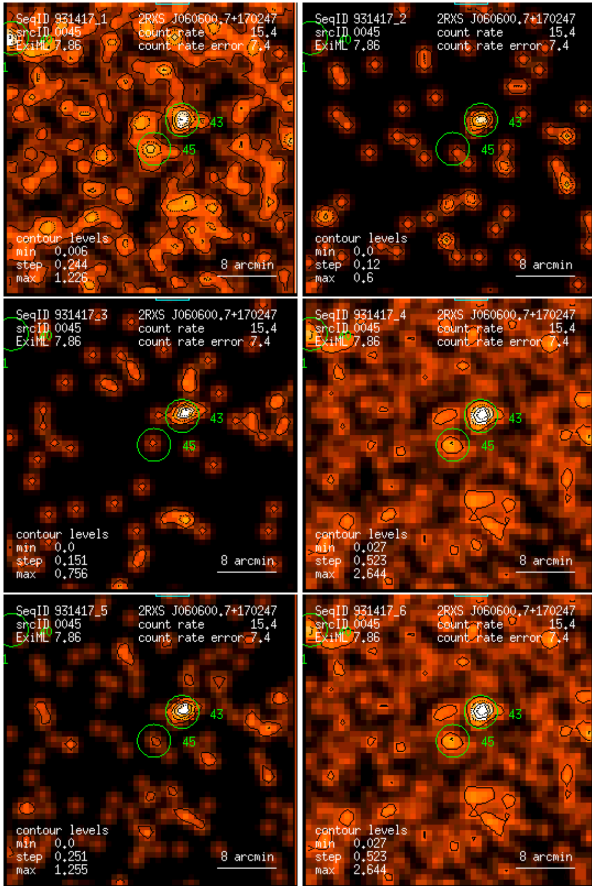
Figure 45: RASS 931417: detection 0045: band rate images, Gaussian filter: (1) PSPC channels 11 – 41, (2) 52 – 90, (3) 91 – 201, (4) 11 – 235, (5) 52 – 201, (6) 11 – 201. Broad band rates in counts/ks. Band rate contour levels in counts/ks/arcmin 2 .
