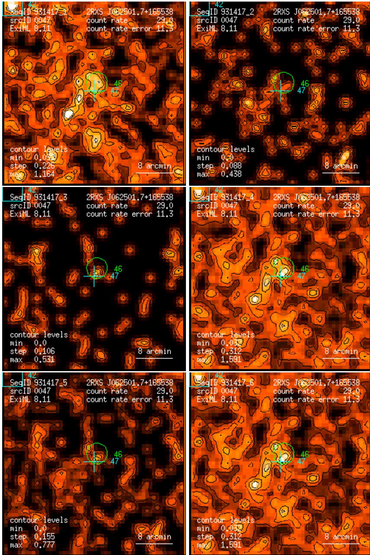
Figure 47: RASS 931417: detection 0047: band rate images, Gaussian filter: (1) PSPC channels 11 – 41, (2) 52 – 90, (3) 91 – 201, (4) 11 – 235, (5) 52 – 201, (6) 11 – 201. Broad band rates in counts/ks. Band rate contour levels in counts/ks/arcmin 2 .
