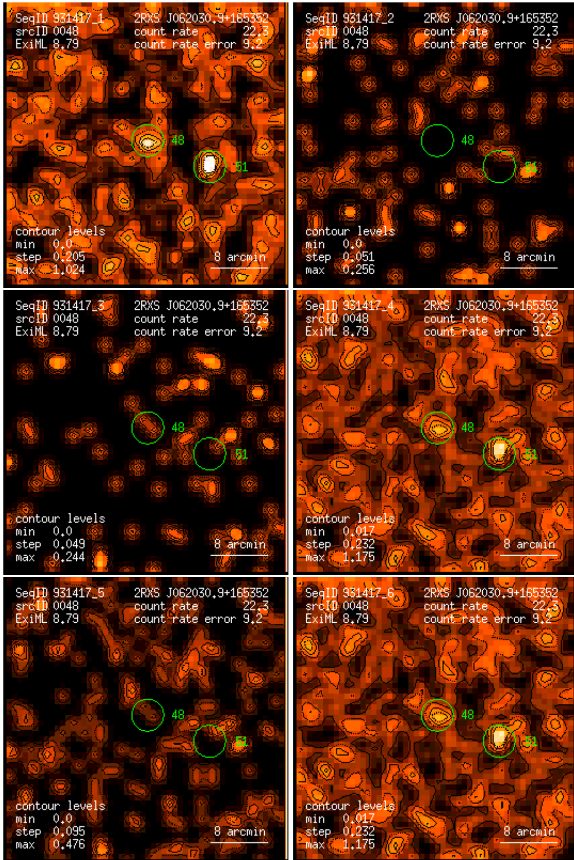
Figure 48: RASS 931417: detection 0048: band rate images, Gaussian filter: (1) PSPC channels 11 – 41, (2) 52 – 90, (3) 91 – 201, (4) 11 – 235, (5) 52 – 201, (6) 11 – 201. Broad band rates in counts/ks. Band rate contour levels in counts/ks/arcmin 2 .
