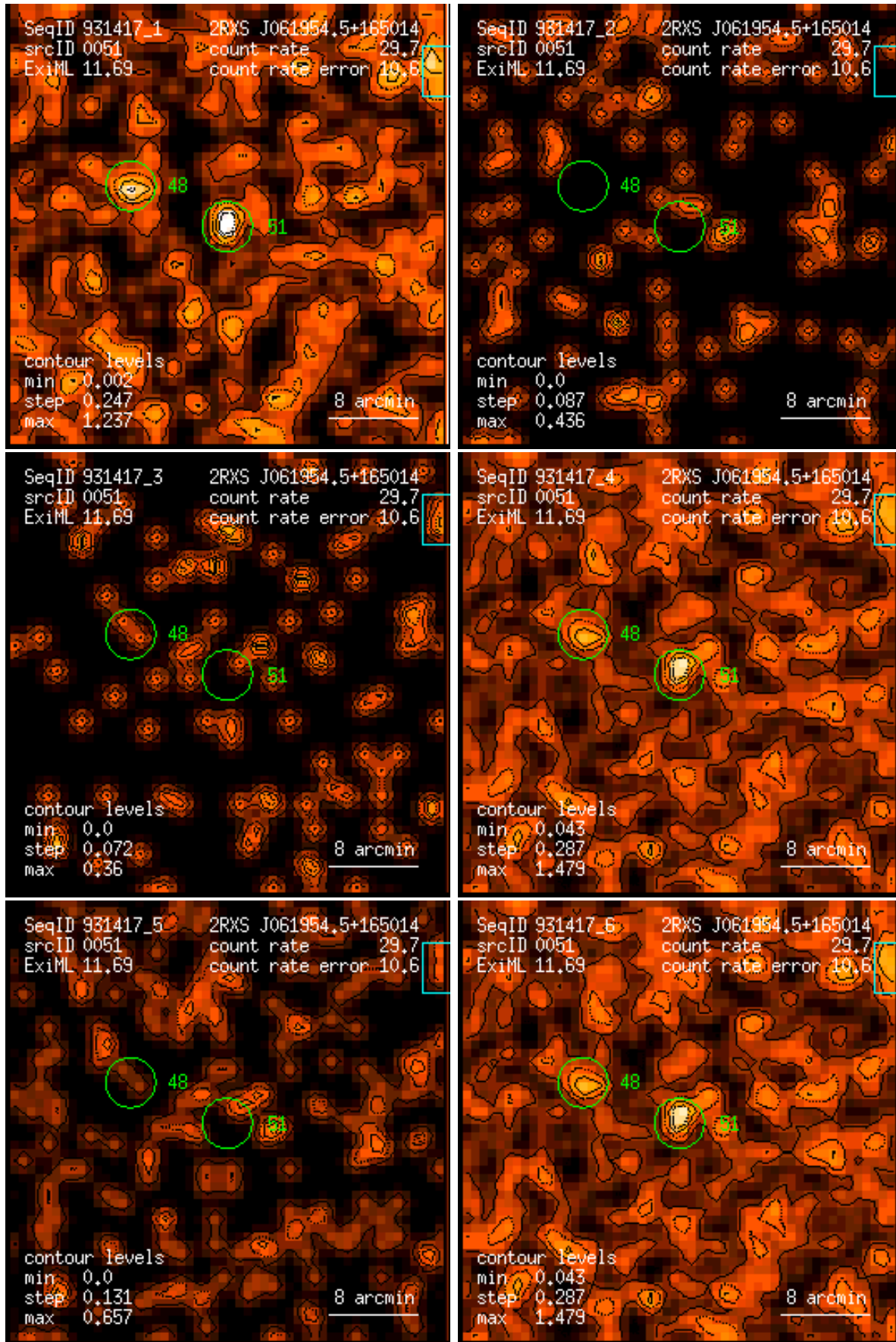
Figure 51: RASS 931417: detection 0051: band rate images, Gaussian filter: (1) PSPC channels 11 – 41, (2) 52 – 90, (3) 91 – 201, (4) 11 – 235, (5) 52 – 201, (6) 11 – 201. Broad band rates in counts/ks. Band rate contour levels in counts/ks/arcmin 2 .
