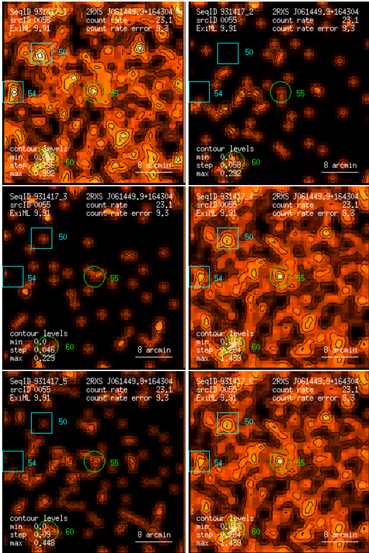
Figure 55: RASS 931417: detection 0055: band rate images, Gaussian filter: (1) PSPC channels 11 – 41, (2) 52 – 90, (3) 91 – 201, (4) 11 – 235, (5) 52 – 201, (6) 11 – 201. Broad band rates in counts/ks. Band rate contour levels in counts/ks/arcmin 2 .
