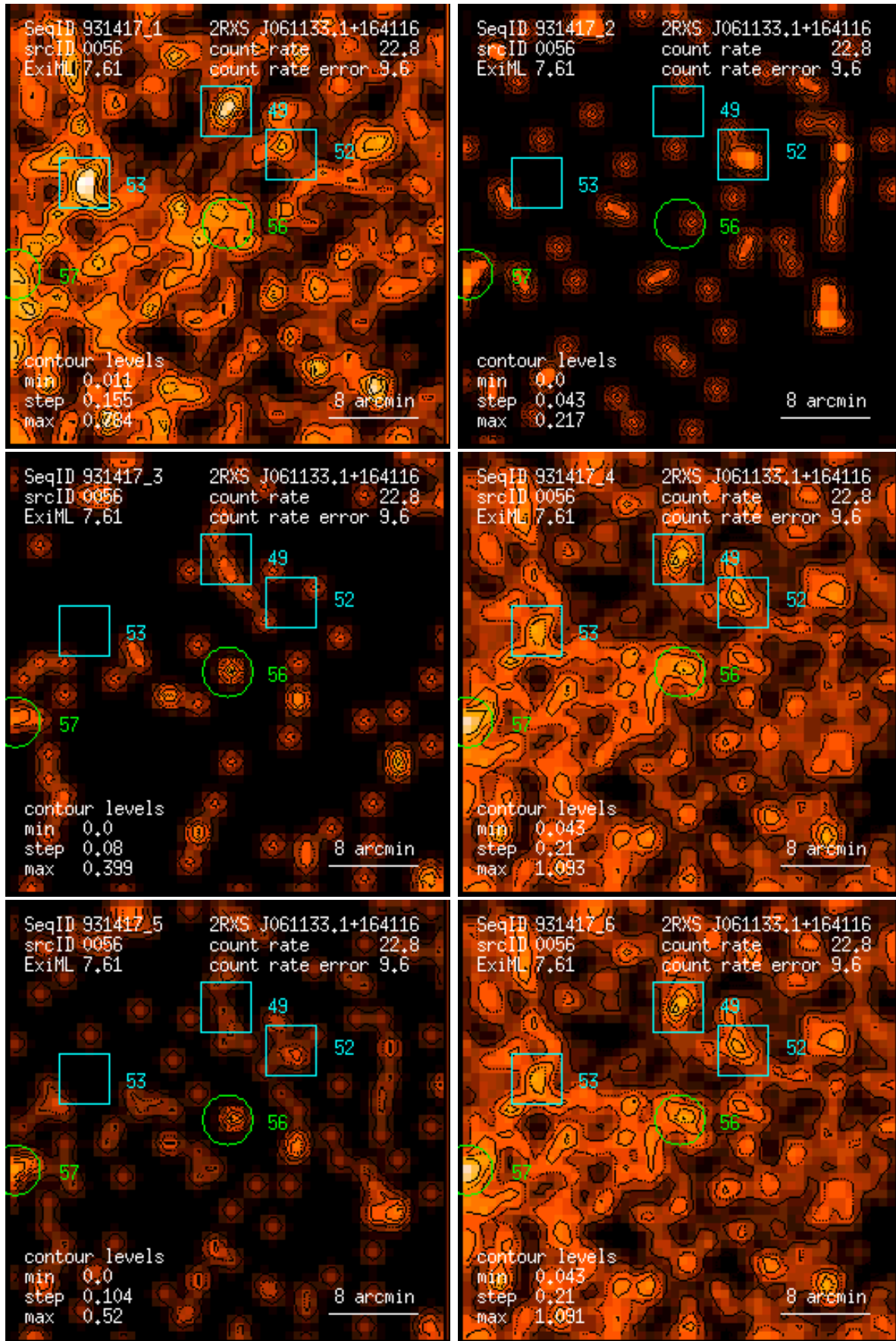
Figure 56: RASS 931417: detection 0056: band rate images, Gaussian filter: (1) PSPC channels 11 – 41, (2) 52 – 90, (3) 91 – 201, (4) 11 – 235, (5) 52 – 201, (6) 11 – 201. Broad band rates in counts/ks. Band rate contour levels in counts/ks/arcmin 2 .
