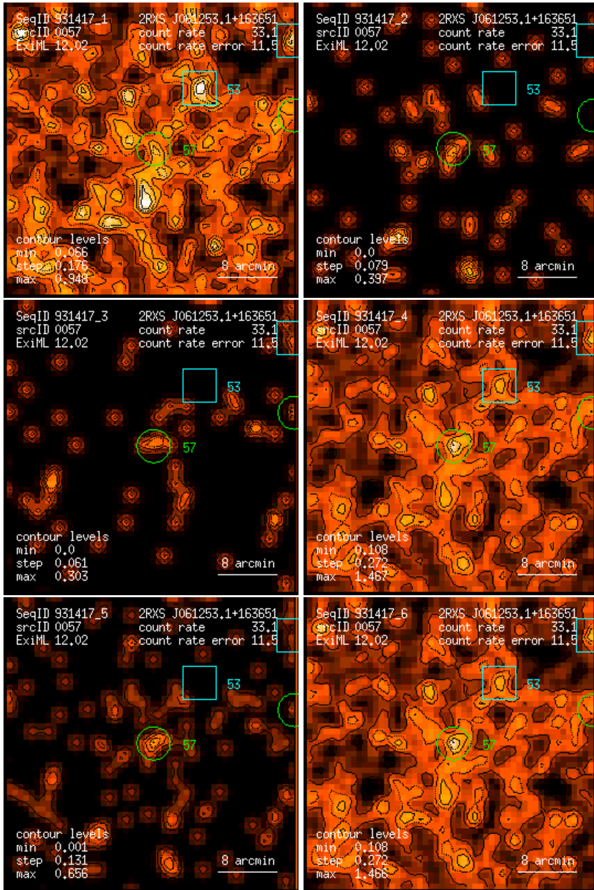
Figure 57: RASS 931417: detection 0057: band rate images, Gaussian filter: (1) PSPC channels 11 – 41, (2) 52 – 90, (3) 91 – 201, (4) 11 – 235, (5) 52 – 201, (6) 11 – 201. Broad band rates in counts/ks. Band rate contour levels in counts/ks/arcmin 2 .
