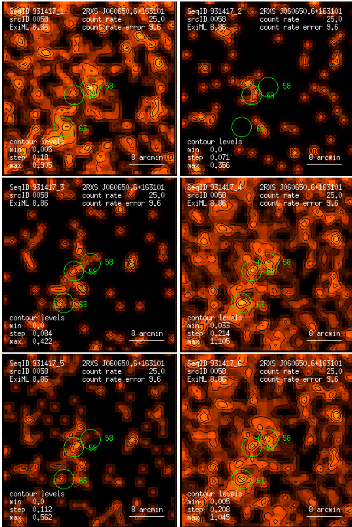
Figure 58: RASS 931417: detection 0058: band rate images, Gaussian filter: (1) PSPC channels 11 – 41, (2) 52 – 90, (3) 91 – 201, (4) 11 – 235, (5) 52 – 201, (6) 11 – 201. Broad band rates in counts/ks. Band rate contour levels in counts/ks/arcmin 2 .
