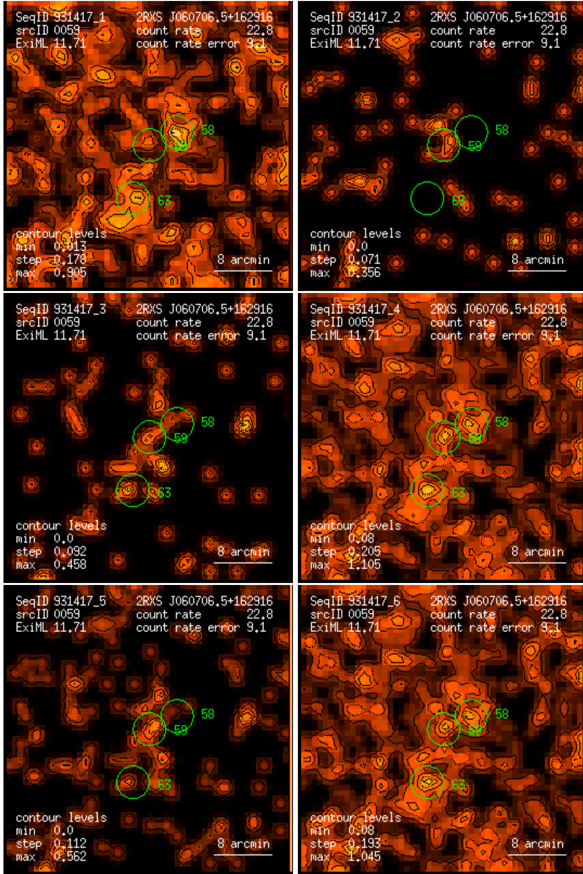
Figure 59: RASS 931417: detection 0059: band rate images, Gaussian filter: (1) PSPC channels 11 – 41, (2) 52 – 90, (3) 91 – 201, (4) 11 – 235, (5) 52 – 201, (6) 11 – 201. Broad band rates in counts/ks. Band rate contour levels in counts/ks/arcmin 2 .
