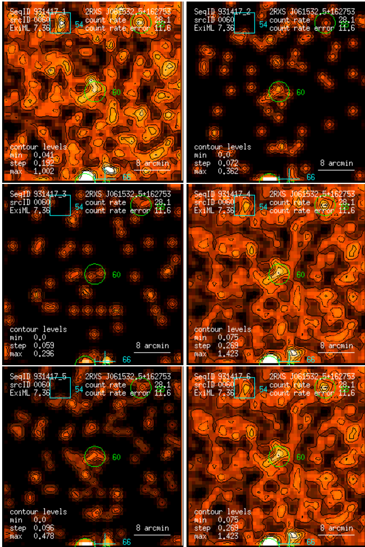
Figure 60: RASS 931417: detection 0060: band rate images, Gaussian filter: (1) PSPC channels 11 – 41, (2) 52 – 90, (3) 91 – 201, (4) 11 – 235, (5) 52 – 201, (6) 11 – 201. Broad band rates in counts/ks. Band rate contour levels in counts/ks/arcmin 2 .
