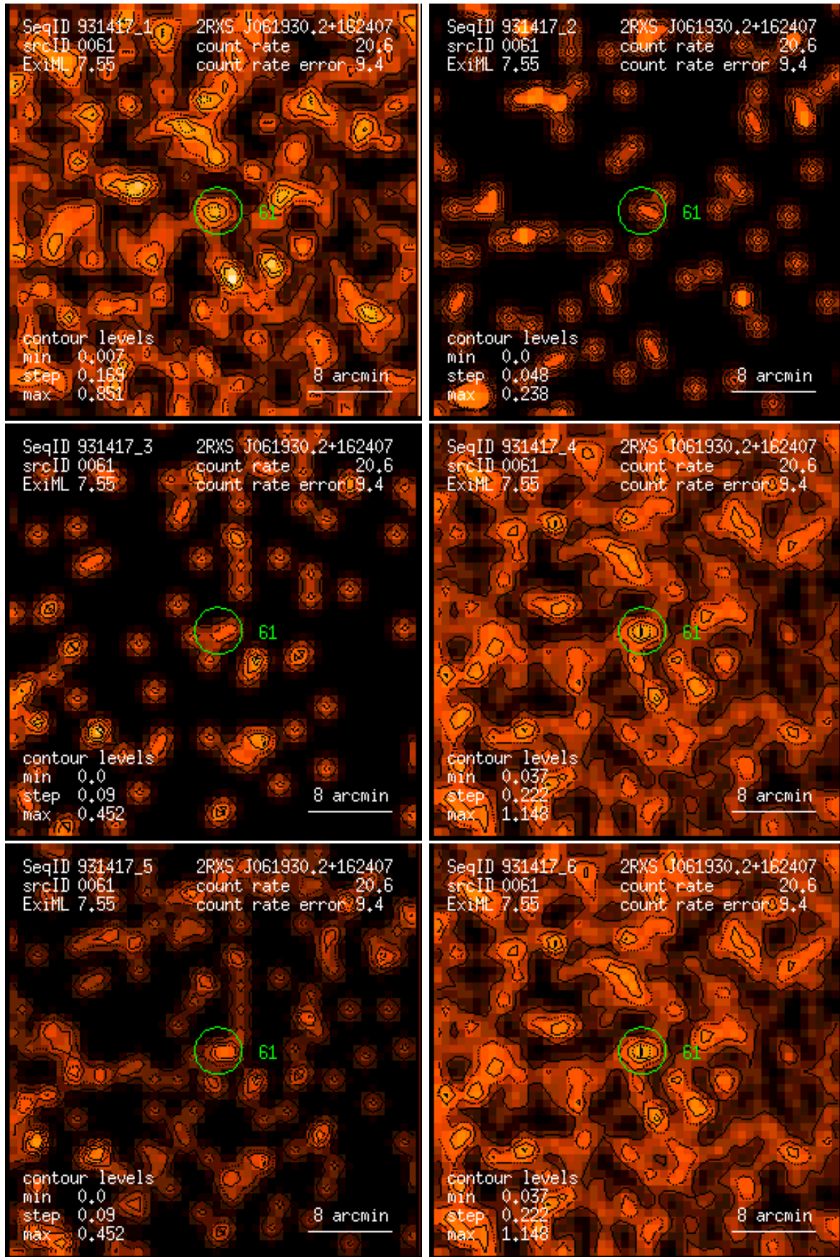
Figure 61: RASS 931417: detection 0061: band rate images, Gaussian filter: (1) PSPC channels 11 – 41, (2) 52 – 90, (3) 91 – 201, (4) 11 – 235, (5) 52 – 201, (6) 11 – 201. Broad band rates in counts/ks. Band rate contour levels in counts/ks/arcmin 2 .
